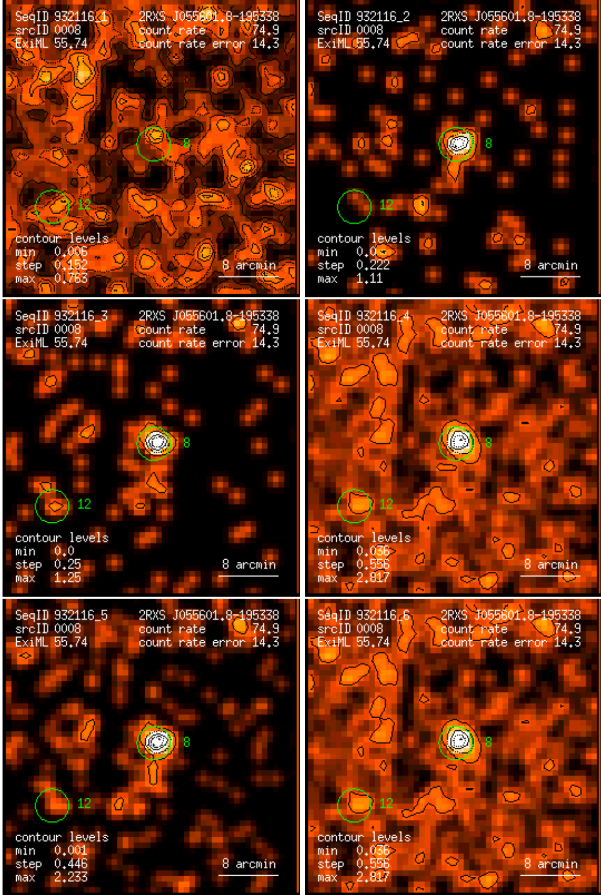
Figure 8: RASS 932116: detection 0008: band rate images, Gaussian filter: (1) PSPC channels 11 – 41, (2) 52 – 90, (3) 91 – 201, (4) 11 – 235, (5) 52 – 201, (6) 11 – 201. Broad band rates in counts/ks. Band rate contour levels in counts/ks/arcmin 2 .
