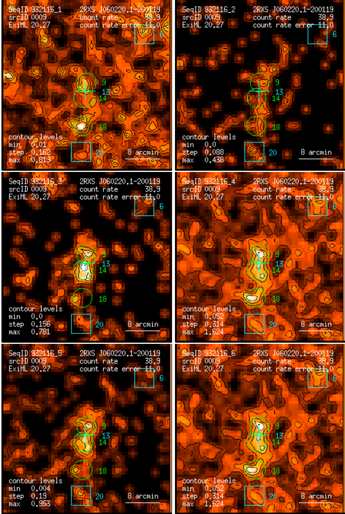
Figure 9: RASS 932116: detection 0009: band rate images, Gaussian filter: (1) PSPC channels 11 – 41, (2) 52 – 90, (3) 91 – 201, (4) 11 – 235, (5) 52 – 201, (6) 11 – 201. Broad band rates in counts/ks. Band rate contour levels in counts/ks/arcmin 2 .
