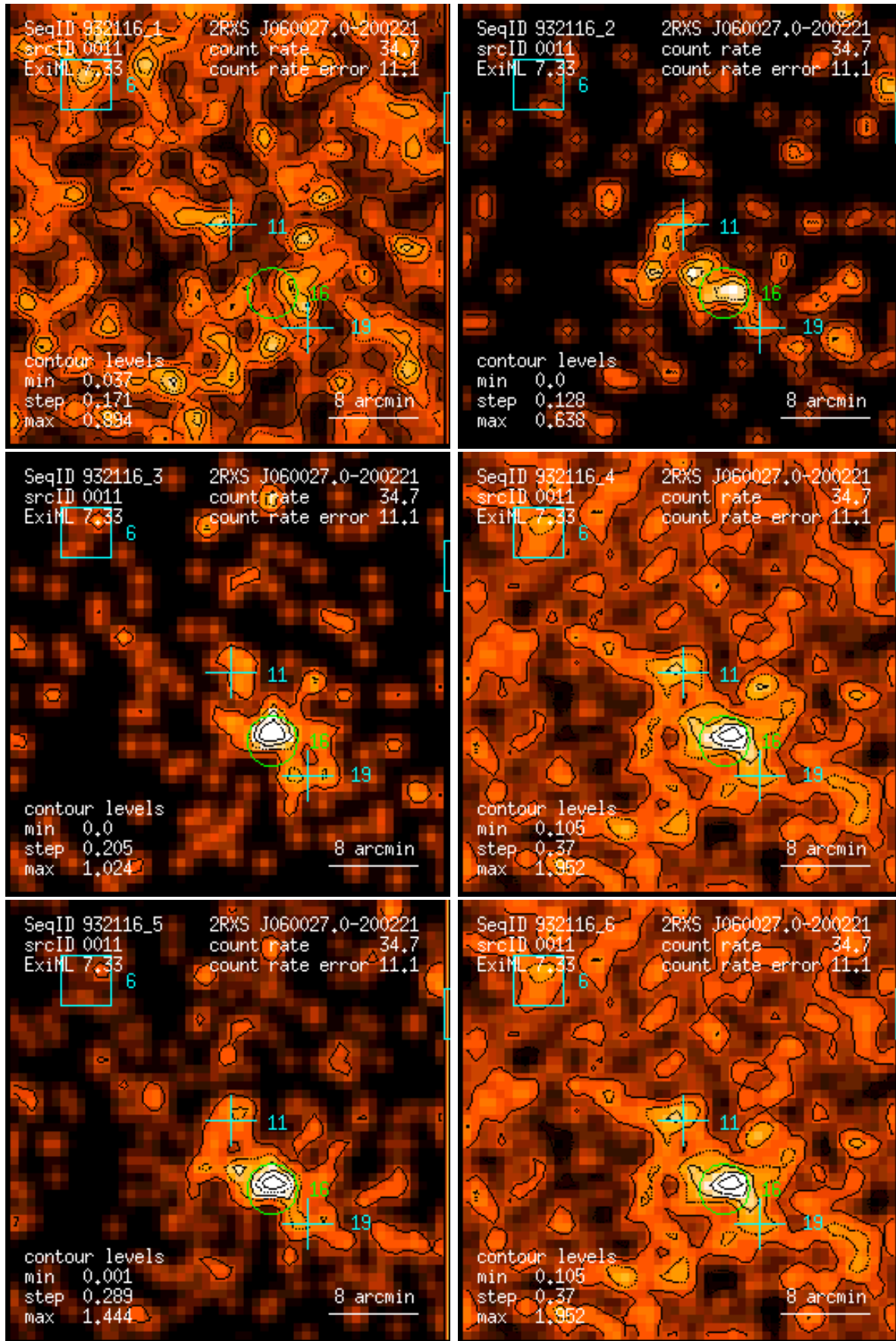
Figure 11: RASS 932116: detection 0011: band rate images, Gaussian filter: (1) PSPC channels 11 – 41, (2) 52 – 90, (3) 91 – 201, (4) 11 – 235, (5) 52 – 201, (6) 11 – 201. Broad band rates in counts/ks. Band rate contour levels in counts/ks/arcmin 2 .
