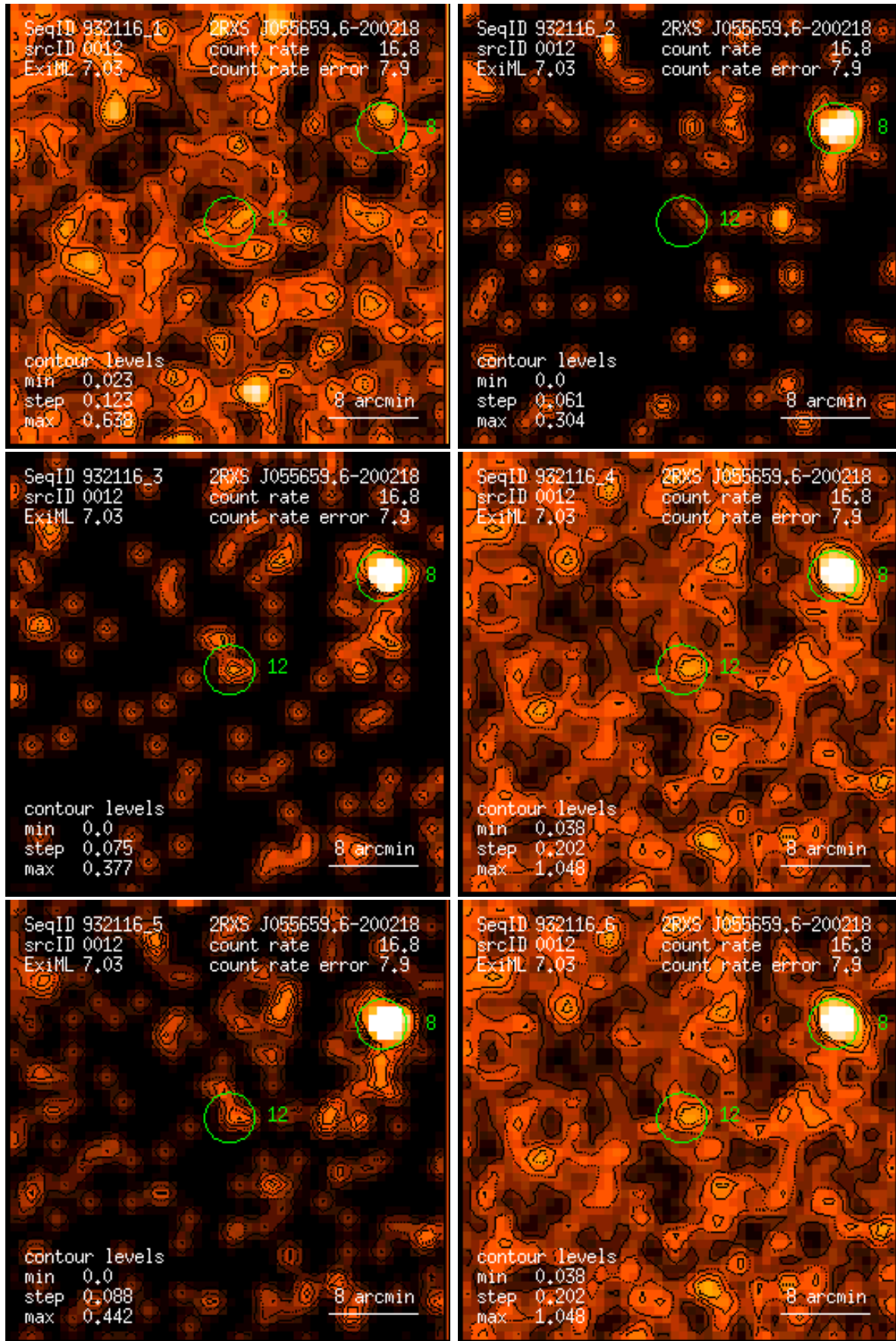
Figure 12: RASS 932116: detection 0012: band rate images, Gaussian filter: (1) PSPC channels 11 – 41, (2) 52 – 90, (3) 91 – 201, (4) 11 – 235, (5) 52 – 201, (6) 11 – 201. Broad band rates in counts/ks. Band rate contour levels in counts/ks/arcmin 2 .
