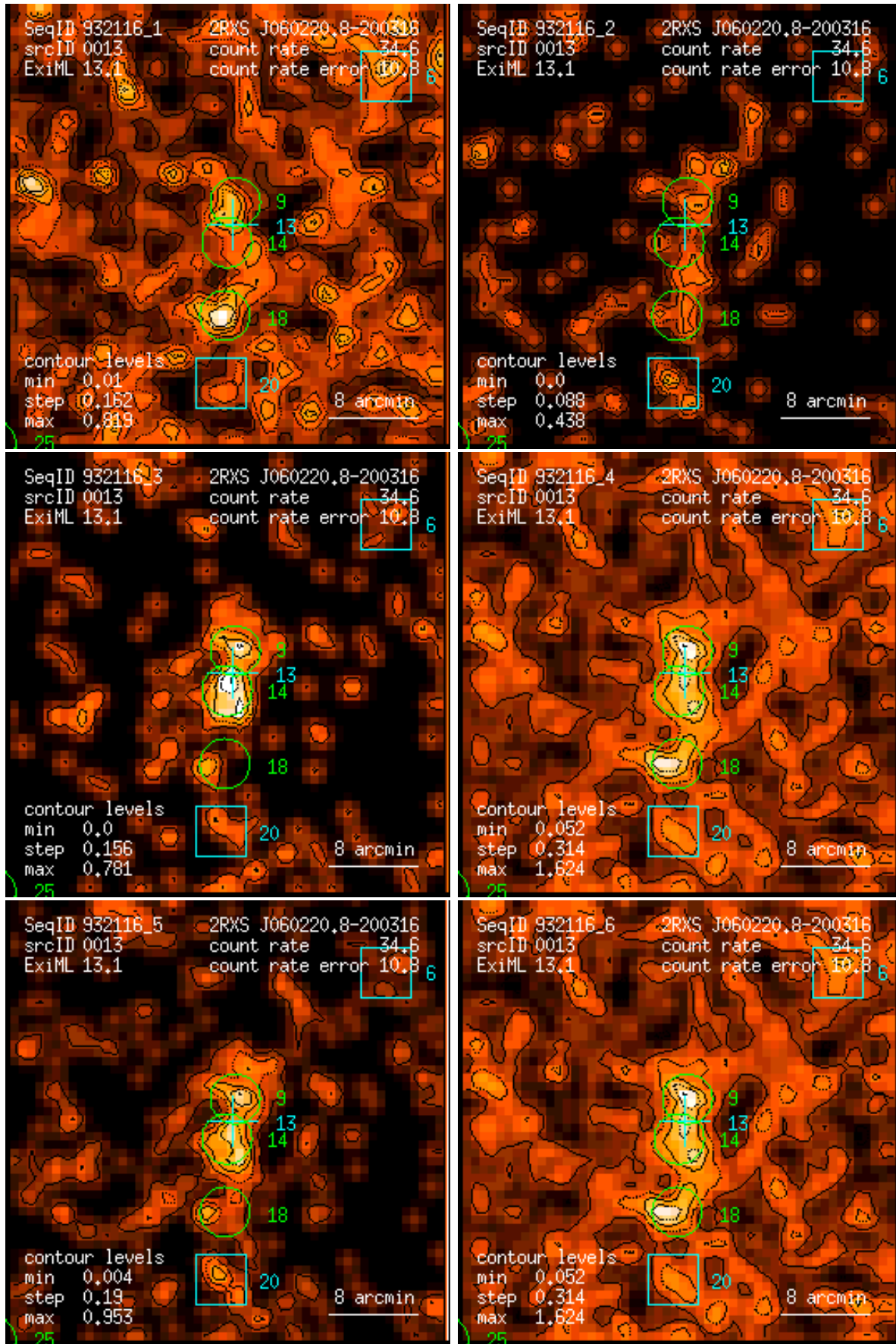
Figure 13: RASS 932116: detection 0013: band rate images, Gaussian filter: (1) PSPC channels 11 – 41, (2) 52 – 90, (3) 91 – 201, (4) 11 – 235, (5) 52 – 201, (6) 11 – 201. Broad band rates in counts/ks. Band rate contour levels in counts/ks/arcmin 2 .
