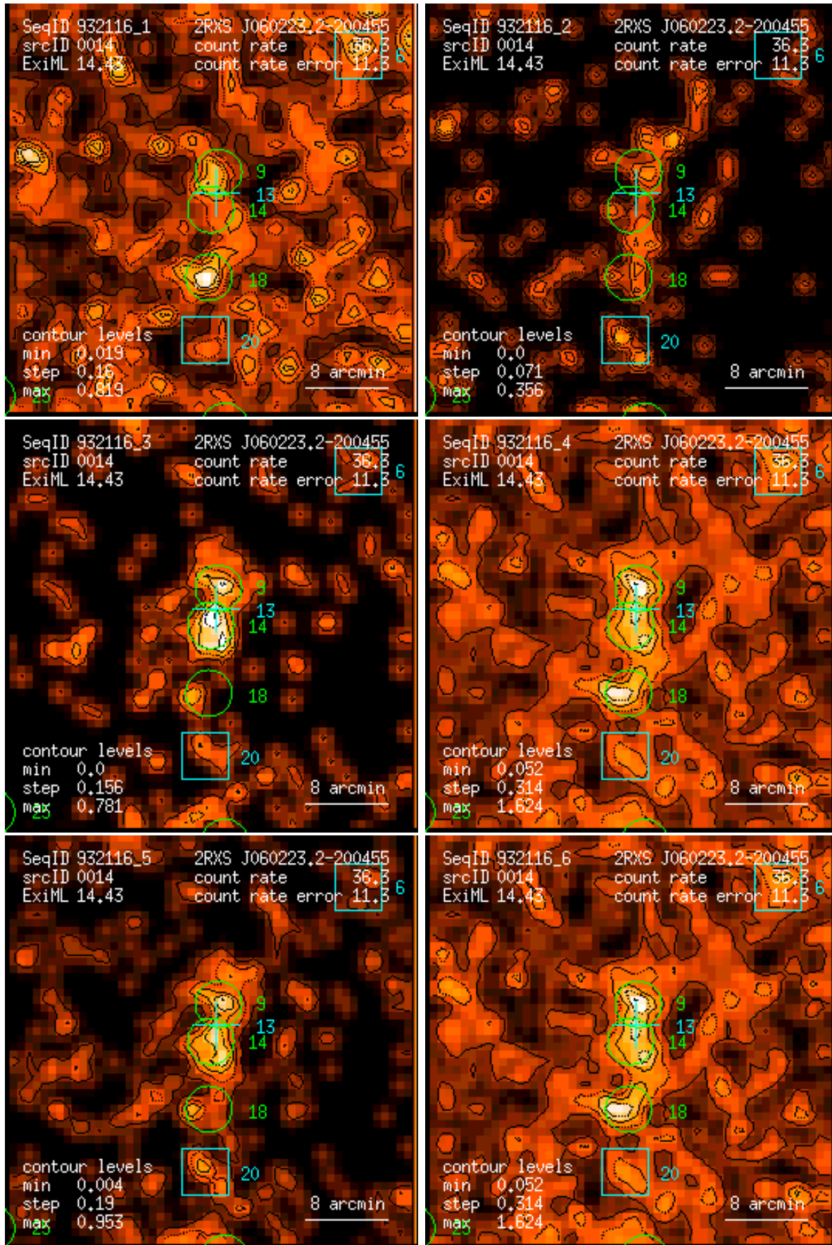
Figure 14: RASS 932116: detection 0014: band rate images, Gaussian filter: (1) PSPC channels 11 – 41, (2) 52 – 90, (3) 91 – 201, (4) 11 – 235, (5) 52 – 201, (6) 11 – 201. Broad band rates in counts/ks. Band rate contour levels in counts/ks/arcmin 2 .
