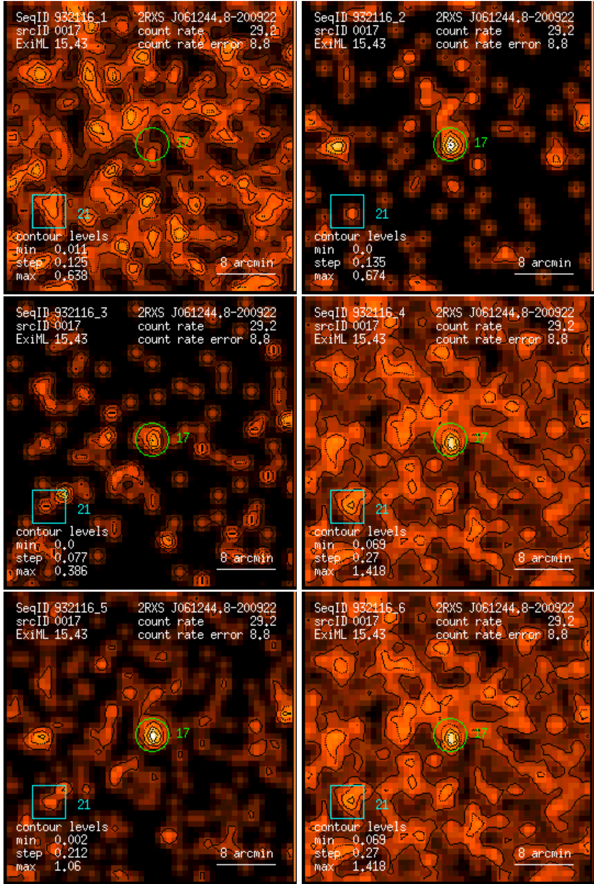
Figure 17: RASS 932116: detection 0017: band rate images, Gaussian filter: (1) PSPC channels 11 – 41, (2) 52 – 90, (3) 91 – 201, (4) 11 – 235, (5) 52 – 201, (6) 11 – 201. Broad band rates in counts/ks. Band rate contour levels in counts/ks/arcmin 2 .
