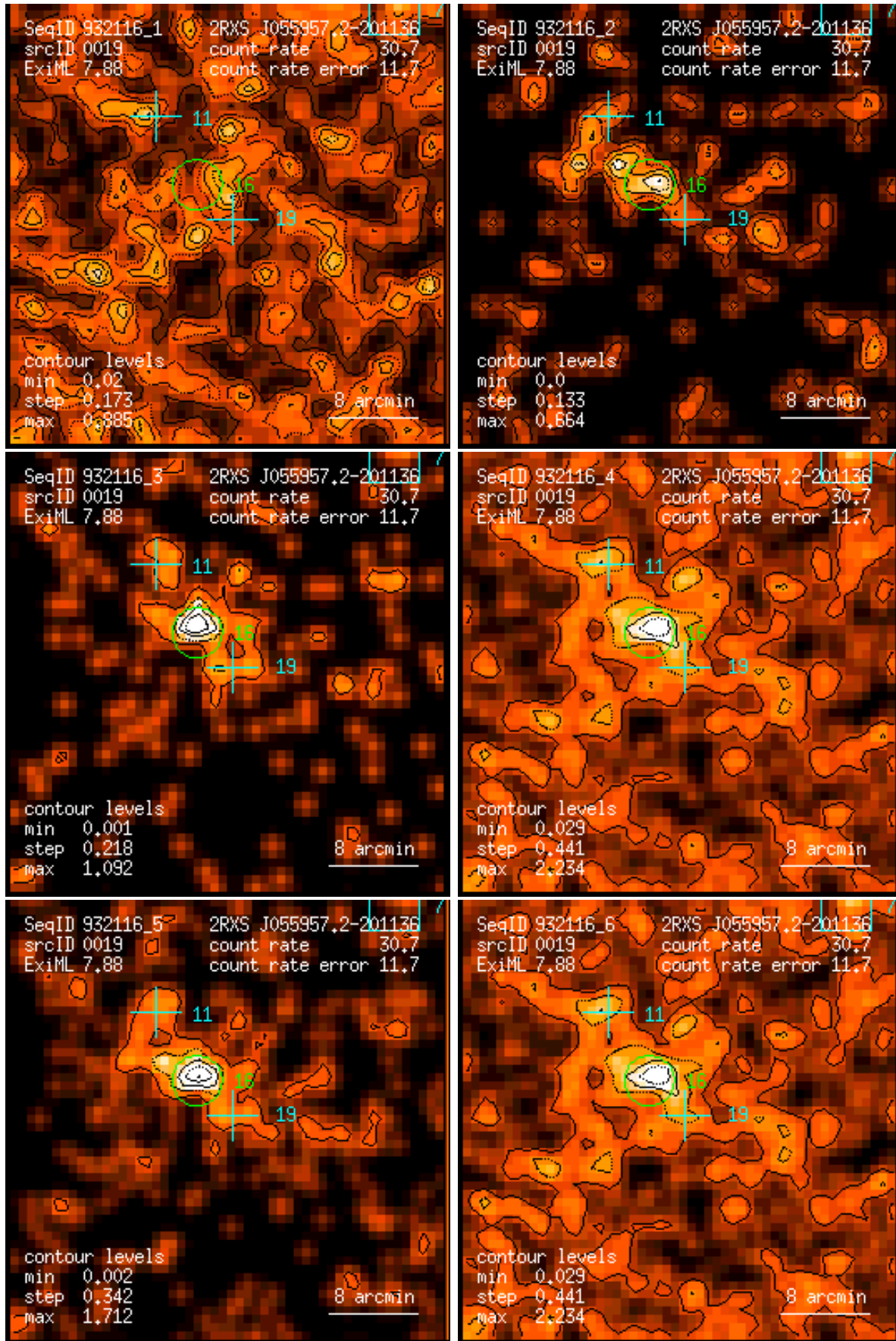
Figure 19: RASS 932116: detection 0019: band rate images, Gaussian filter: (1) PSPC channels 11 – 41, (2) 52 – 90, (3) 91 – 201, (4) 11 – 235, (5) 52 – 201, (6) 11 – 201. Broad band rates in counts/ks. Band rate contour levels in counts/ks/arcmin 2 .
