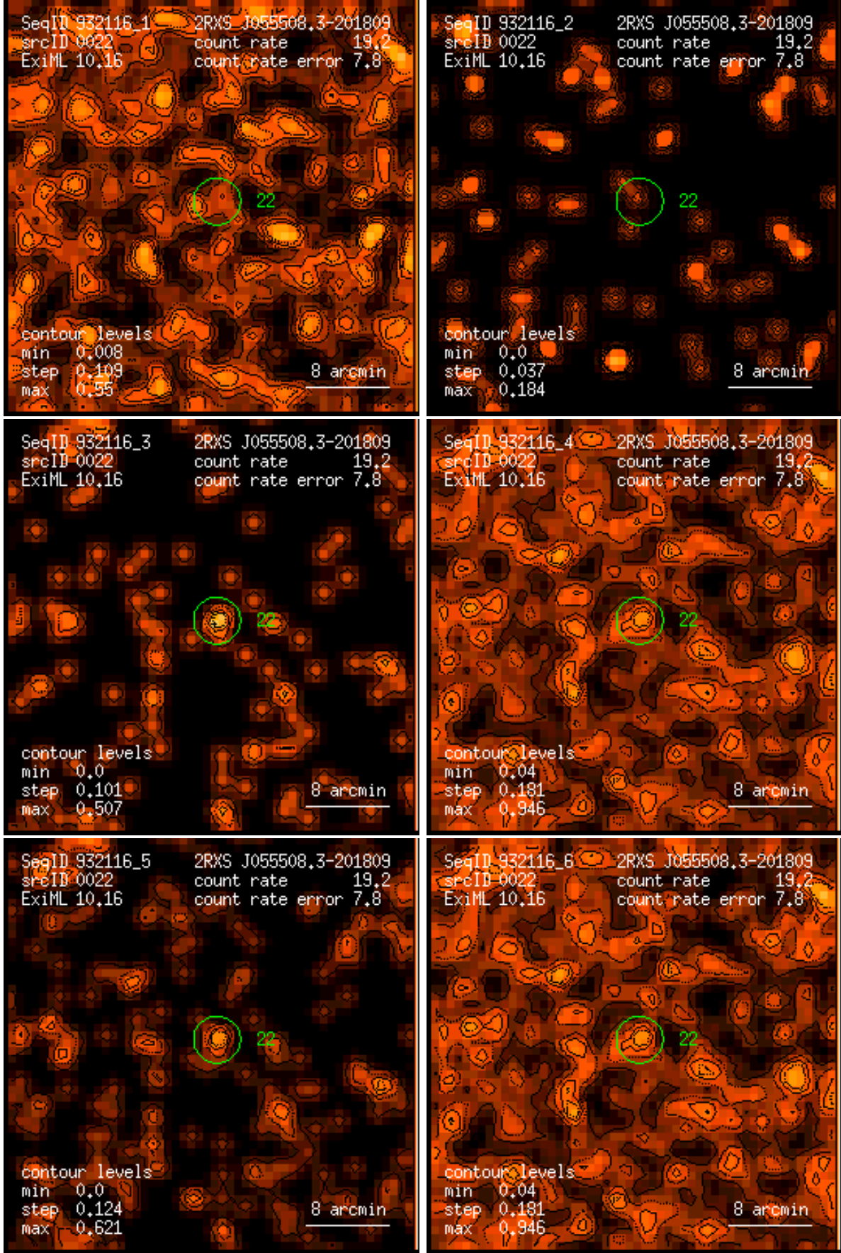
Figure 22: RASS 932116: detection 0022: band rate images, Gaussian filter: (1) PSPC channels 11 – 41, (2) 52 – 90, (3) 91 – 201, (4) 11 – 235, (5) 52 – 201, (6) 11 – 201. Broad band rates in counts/ks. Band rate contour levels in counts/ks/arcmin 2 .
