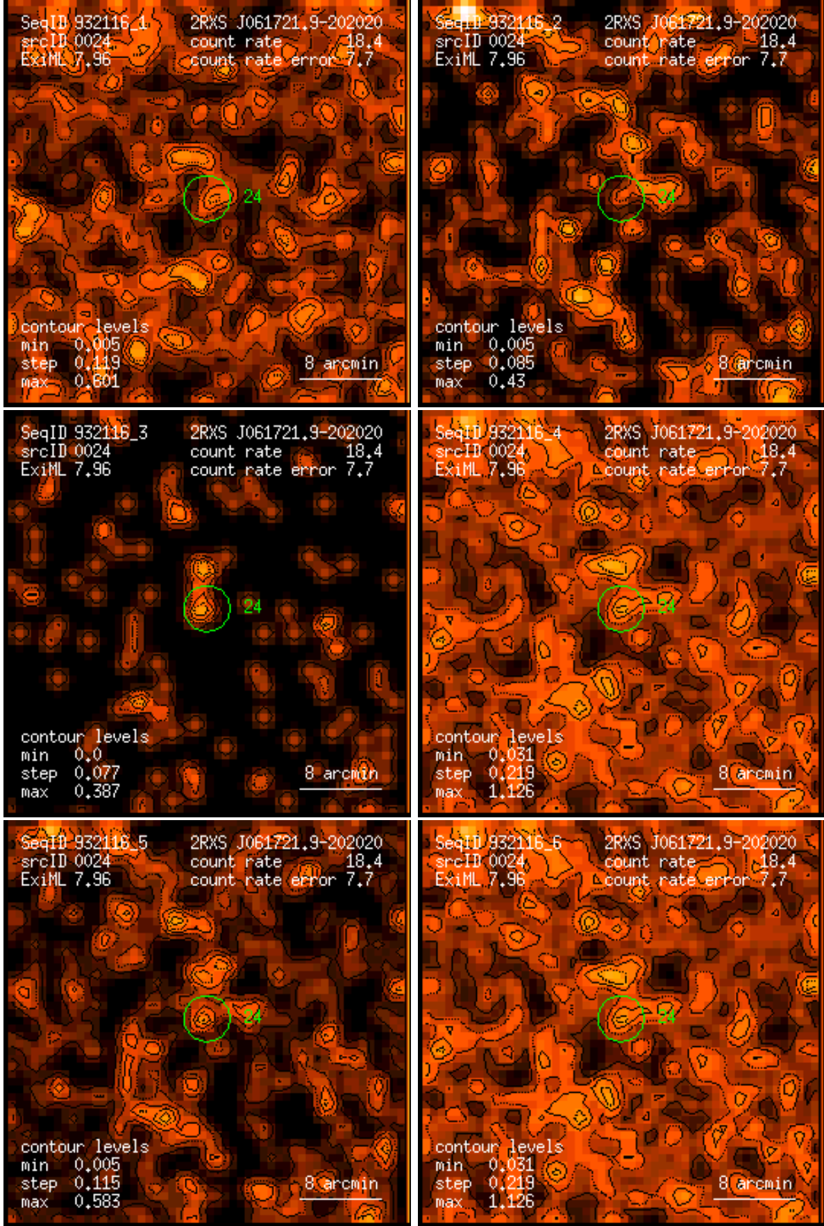
Figure 24: RASS 932116: detection 0024: band rate images, Gaussian filter: (1) PSPC channels 11 – 41, (2) 52 – 90, (3) 91 – 201, (4) 11 – 235, (5) 52 – 201, (6) 11 – 201. Broad band rates in counts/ks. Band rate contour levels in counts/ks/arcmin 2 .
