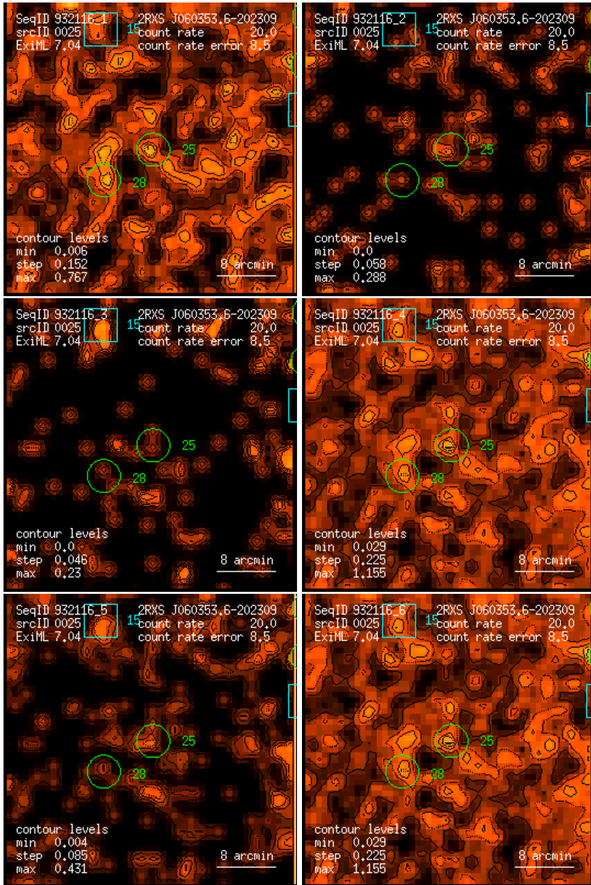
Figure 25: RASS 932116: detection 0025: band rate images, Gaussian filter: (1) PSPC channels 11 – 41, (2) 52 – 90, (3) 91 – 201, (4) 11 – 235, (5) 52 – 201, (6) 11 – 201. Broad band rates in counts/ks. Band rate contour levels in counts/ks/arcmin 2 .
