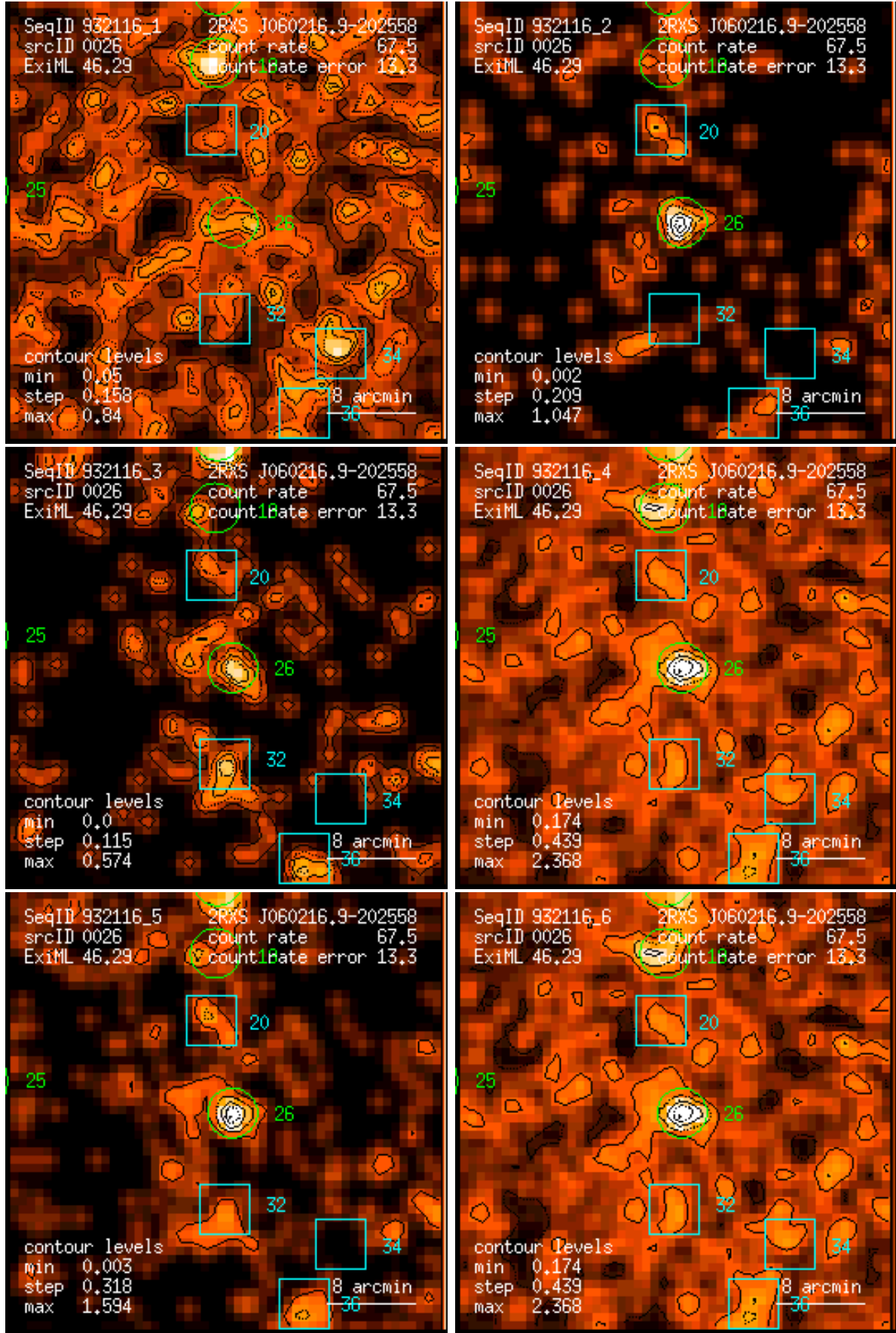
Figure 26: RASS 932116: detection 0026: band rate images, Gaussian filter: (1) PSPC channels 11 – 41, (2) 52 – 90, (3) 91 – 201, (4) 11 – 235, (5) 52 – 201, (6) 11 – 201. Broad band rates in counts/ks. Band rate contour levels in counts/ks/arcmin 2 .
