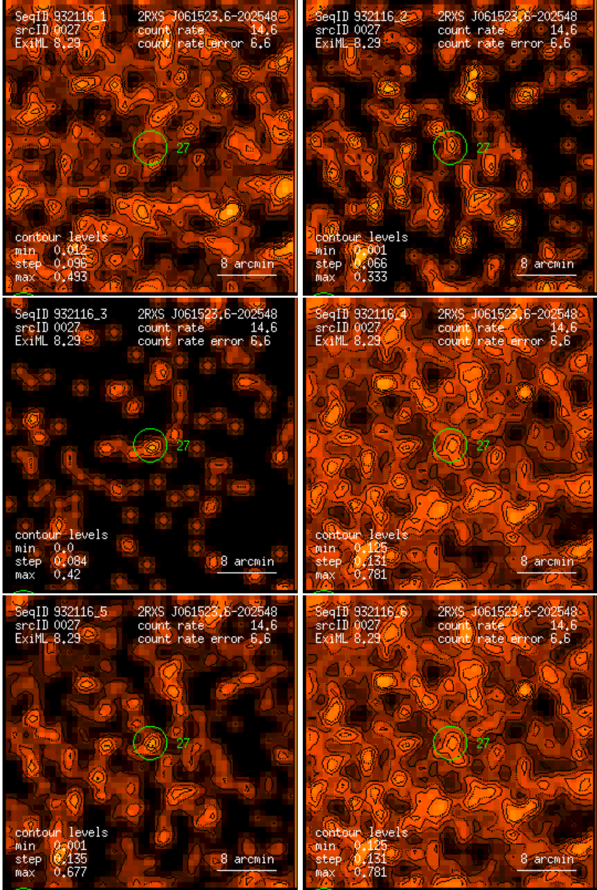
Figure 27: RASS 932116: detection 0027: band rate images, Gaussian filter: (1) PSPC channels 11 – 41, (2) 52 – 90, (3) 91 – 201, (4) 11 – 235, (5) 52 – 201, (6) 11 – 201. Broad band rates in counts/ks. Band rate contour levels in counts/ks/arcmin 2 .
