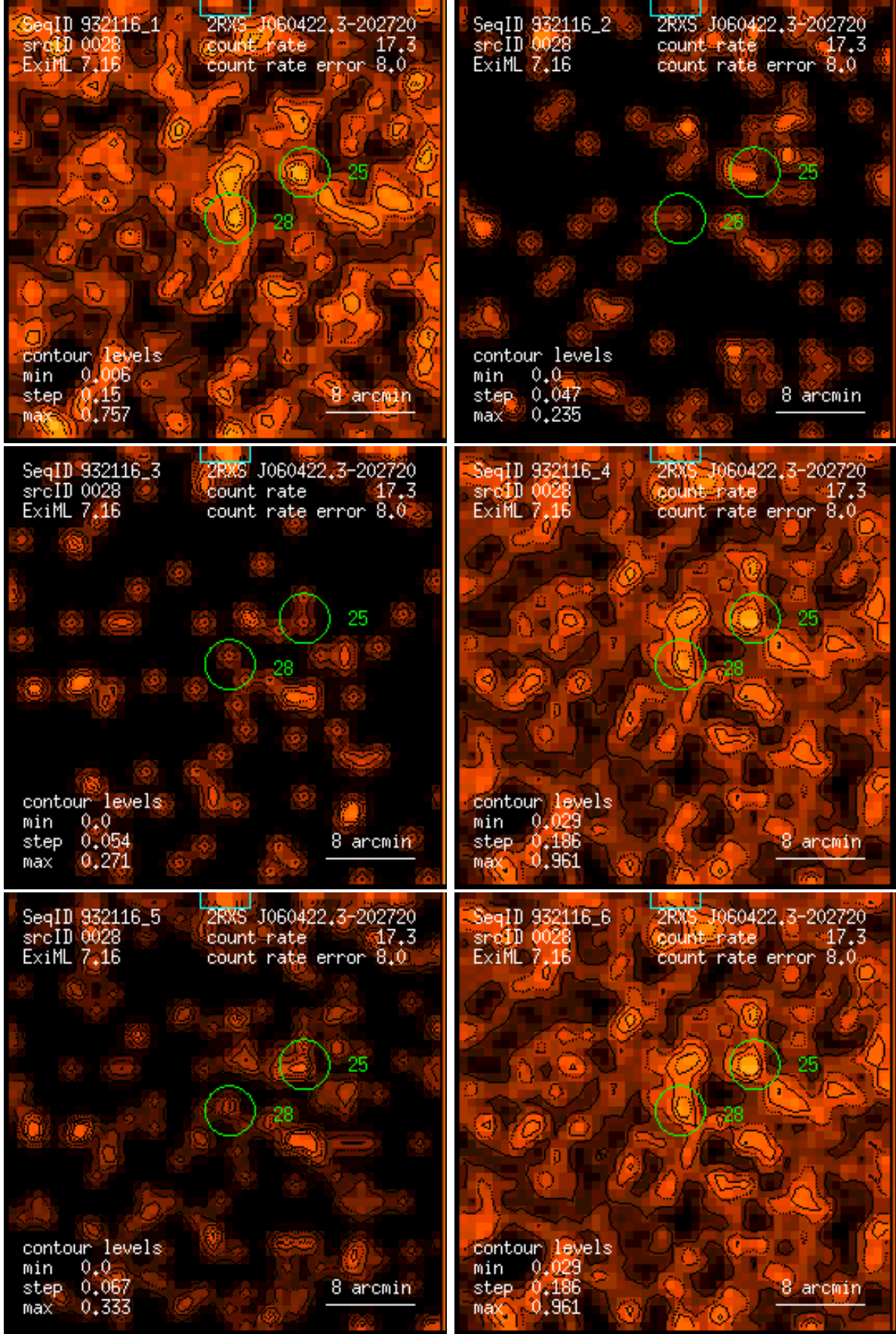
Figure 28: RASS 932116: detection 0028: band rate images, Gaussian filter: (1) PSPC channels 11 – 41, (2) 52 – 90, (3) 91 – 201, (4) 11 – 235, (5) 52 – 201, (6) 11 – 201. Broad band rates in counts/ks. Band rate contour levels in counts/ks/arcmin 2 .
