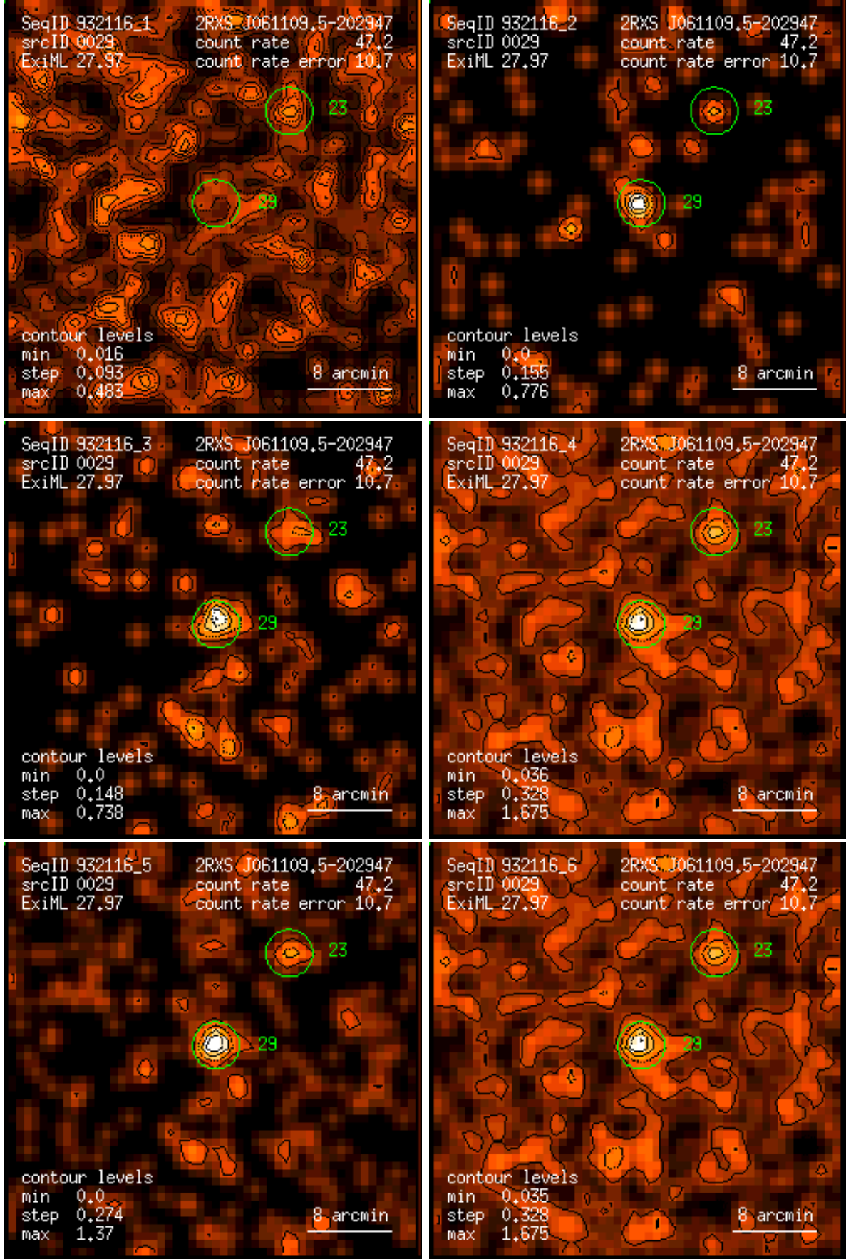
Figure 29: RASS 932116: detection 0029: band rate images, Gaussian filter: (1) PSPC channels 11 – 41, (2) 52 – 90, (3) 91 – 201, (4) 11 – 235, (5) 52 – 201, (6) 11 – 201. Broad band rates in counts/ks. Band rate contour levels in counts/ks/arcmin 2 .
