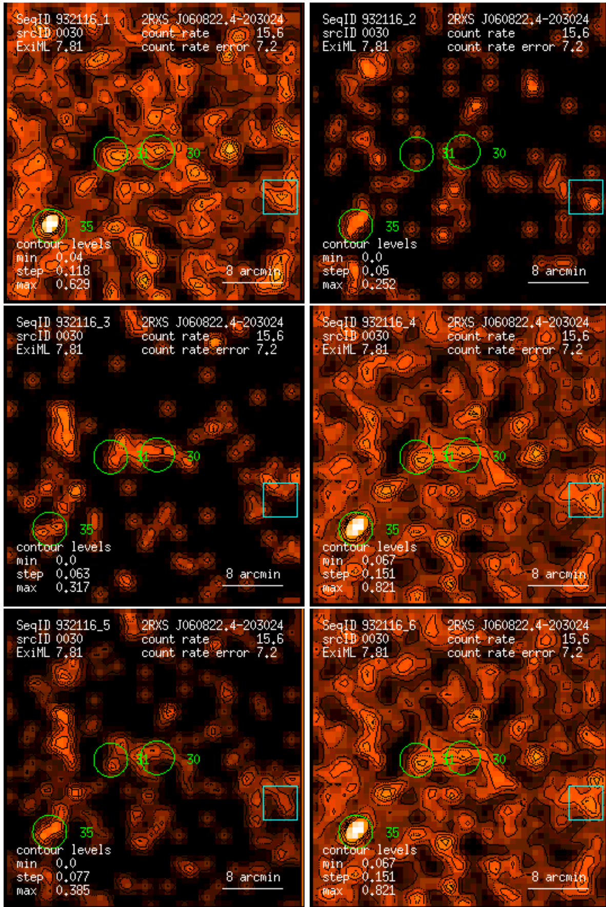
Figure 30: RASS 932116: detection 0030: band rate images, Gaussian filter: (1) PSPC channels 11 – 41, (2) 52 – 90, (3) 91 – 201, (4) 11 – 235, (5) 52 – 201, (6) 11 – 201. Broad band rates in counts/ks. Band rate contour levels in counts/ks/arcmin 2 .
