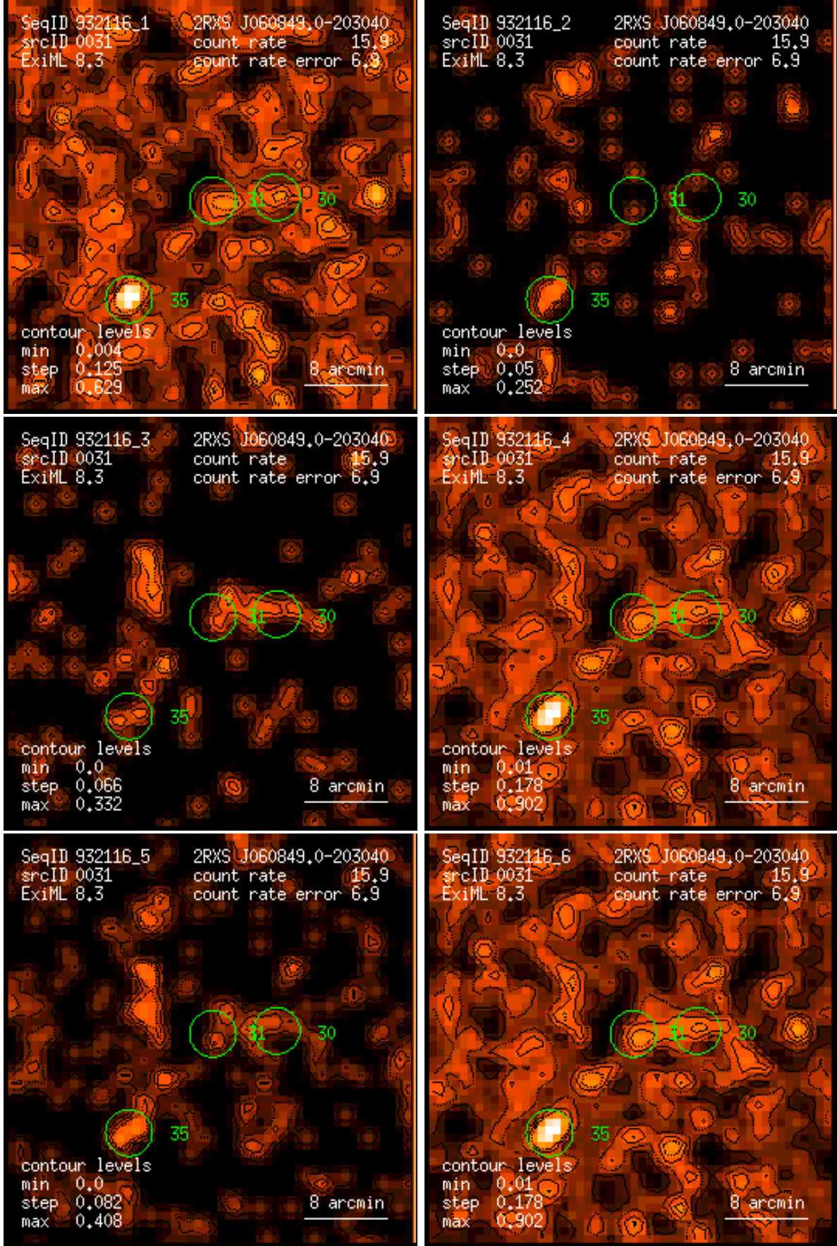
Figure 31: RASS 932116: detection 0031: band rate images, Gaussian filter: (1) PSPC channels 11 – 41, (2) 52 – 90, (3) 91 – 201, (4) 11 – 235, (5) 52 – 201, (6) 11 – 201. Broad band rates in counts/ks. Band rate contour levels in counts/ks/arcmin 2 .
