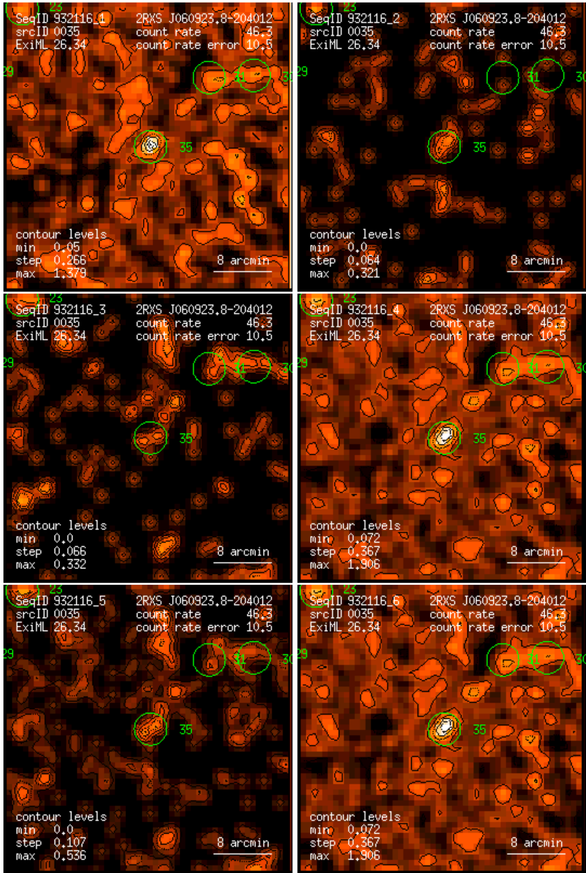
Figure 35: RASS 932116: detection 0035: band rate images, Gaussian filter: (1) PSPC channels 11 – 41, (2) 52 – 90, (3) 91 – 201, (4) 11 – 235, (5) 52 – 201, (6) 11 – 201. Broad band rates in counts/ks. Band rate contour levels in counts/ks/arcmin 2 .
