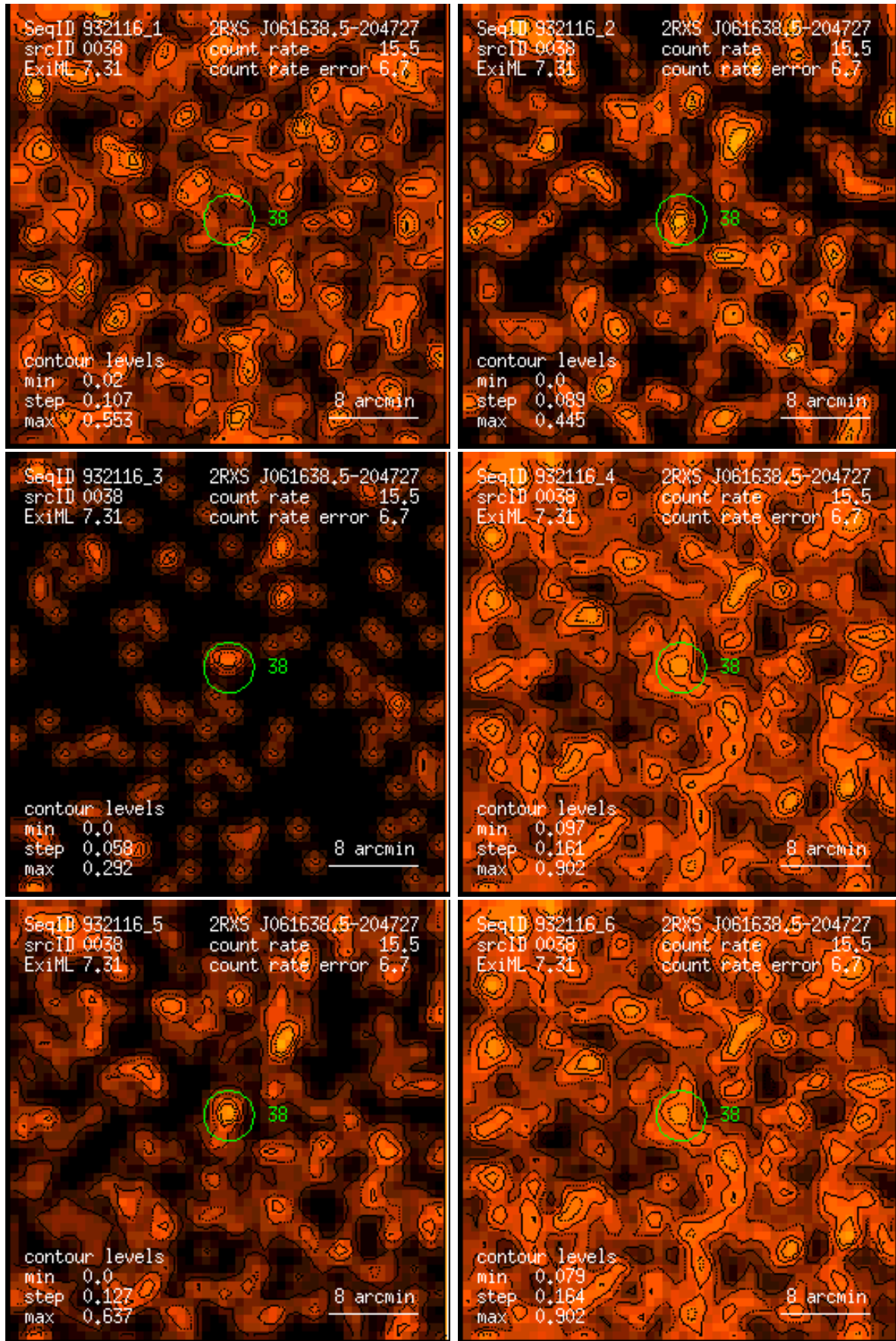
Figure 38: RASS 932116: detection 0038: band rate images, Gaussian filter: (1) PSPC channels 11 – 41, (2) 52 – 90, (3) 91 – 201, (4) 11 – 235, (5) 52 – 201, (6) 11 – 201. Broad band rates in counts/ks. Band rate contour levels in counts/ks/arcmin 2 .
