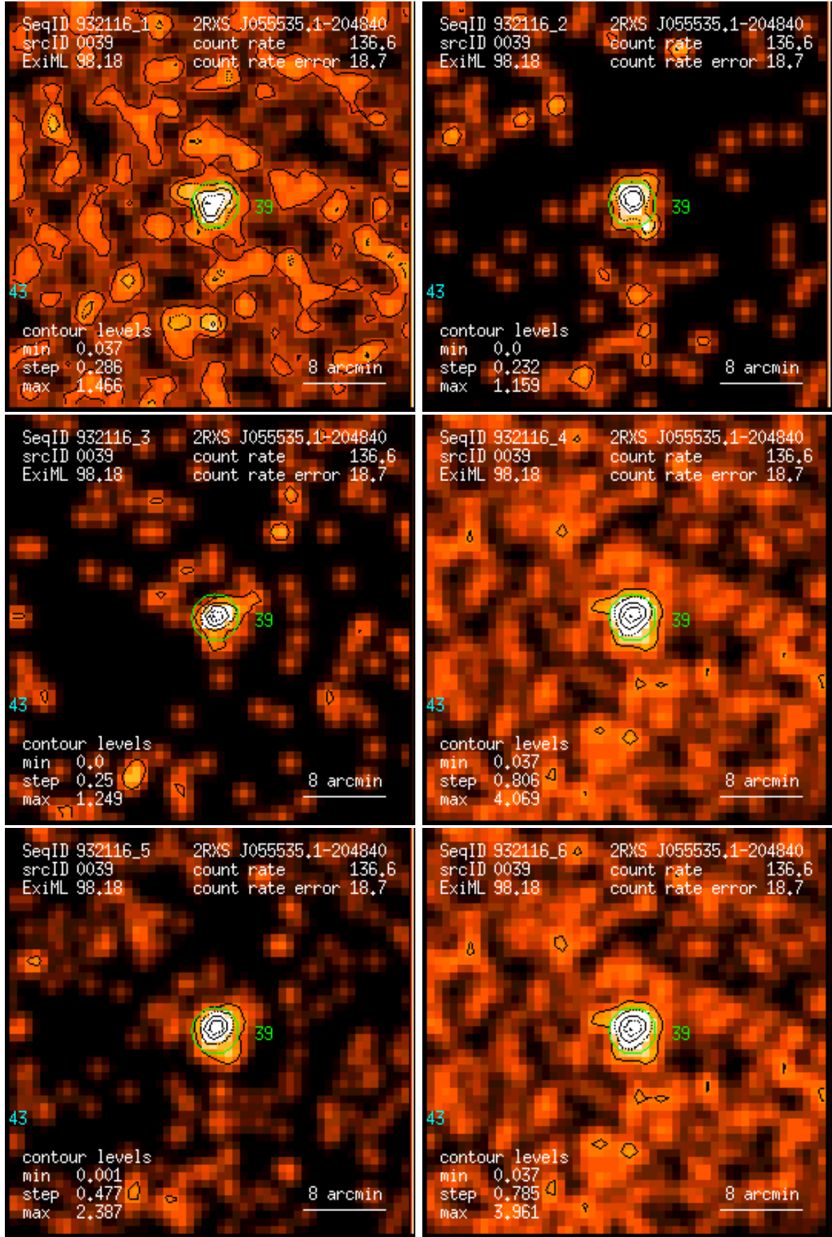
Figure 39: RASS 932116: detection 0039: band rate images, Gaussian filter: (1) PSPC channels 11 – 41, (2) 52 – 90, (3) 91 – 201, (4) 11 – 235, (5) 52 – 201, (6) 11 – 201. Broad band rates in counts/ks. Band rate contour levels in counts/ks/arcmin 2 .
