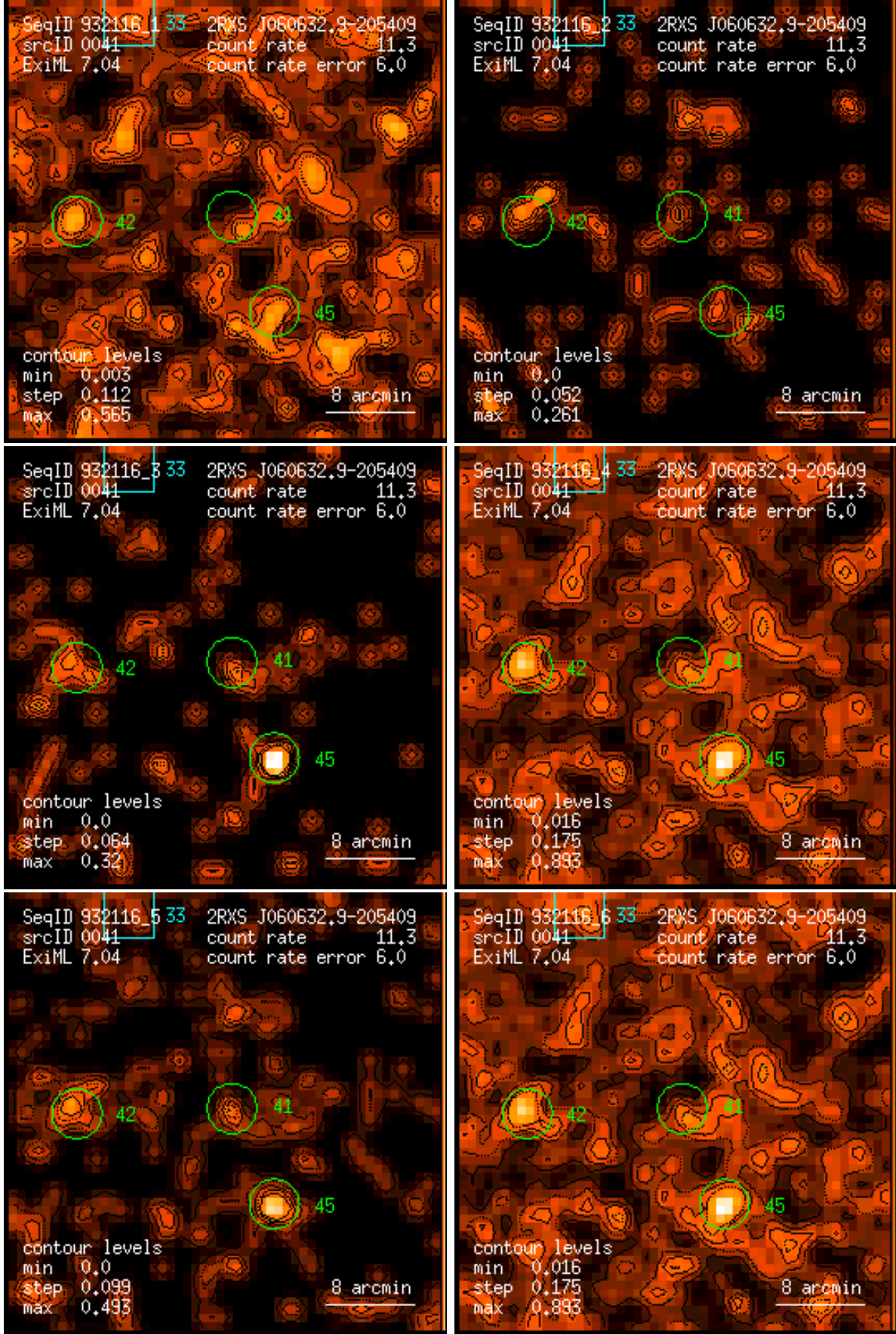
Figure 41: RASS 932116: detection 0041: band rate images, Gaussian filter: (1) PSPC channels 11 – 41, (2) 52 – 90, (3) 91 – 201, (4) 11 – 235, (5) 52 – 201, (6) 11 – 201. Broad band rates in counts/ks. Band rate contour levels in counts/ks/arcmin 2 .
