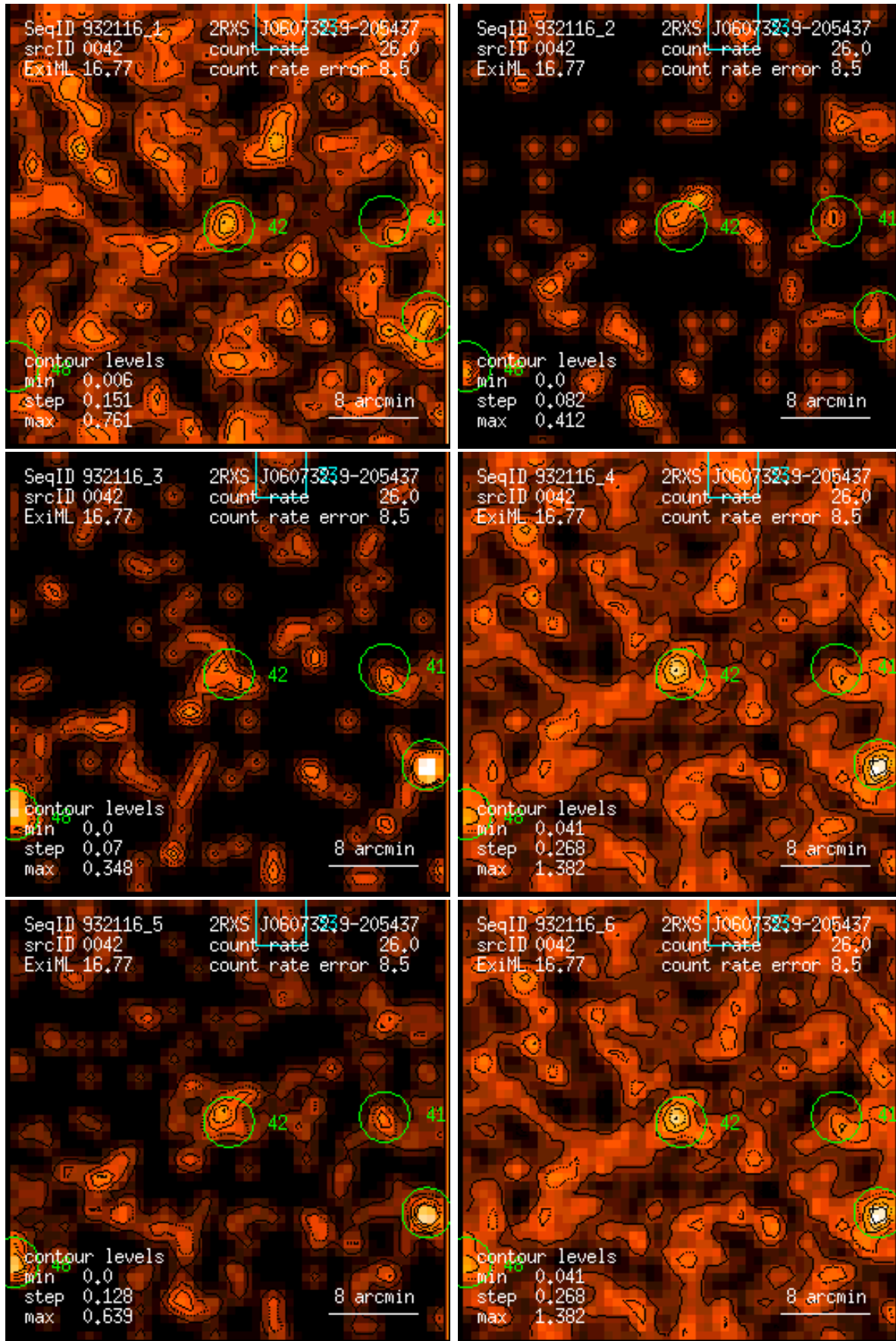
Figure 42: RASS 932116: detection 0042: band rate images, Gaussian filter: (1) PSPC channels 11 – 41, (2) 52 – 90, (3) 91 – 201, (4) 11 – 235, (5) 52 – 201, (6) 11 – 201. Broad band rates in counts/ks. Band rate contour levels in counts/ks/arcmin 2 .
