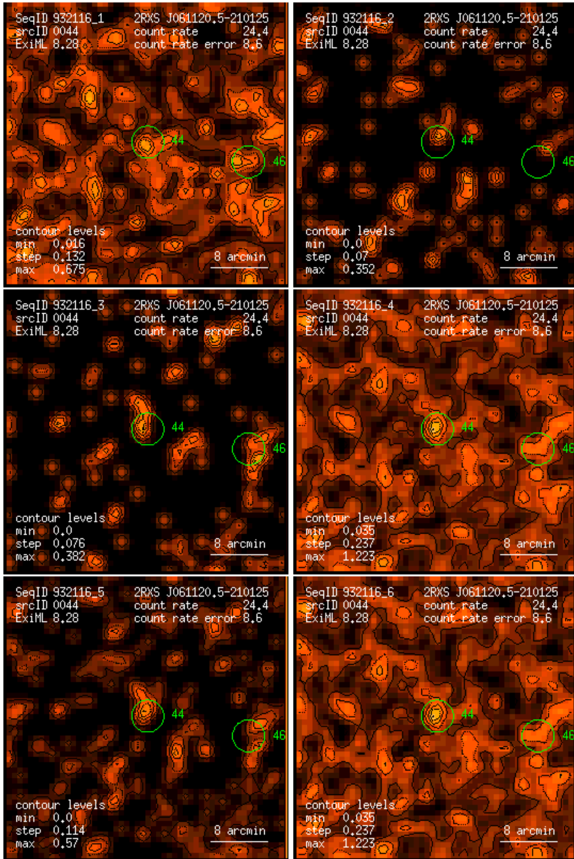
Figure 44: RASS 932116: detection 0044: band rate images, Gaussian filter: (1) PSPC channels 11 – 41, (2) 52 – 90, (3) 91 – 201, (4) 11 – 235, (5) 52 – 201, (6) 11 – 201. Broad band rates in counts/ks. Band rate contour levels in counts/ks/arcmin 2 .
