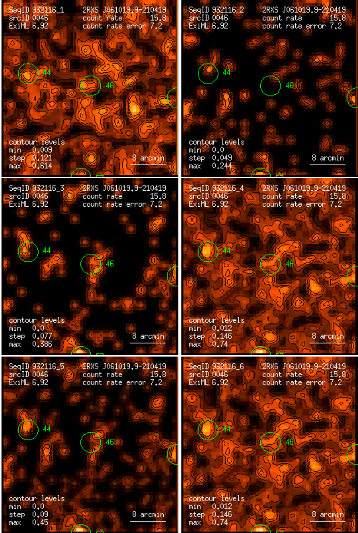
Figure 46: RASS 932116: detection 0046: band rate images, Gaussian filter: (1) PSPC channels 11 – 41, (2) 52 – 90, (3) 91 – 201, (4) 11 – 235, (5) 52 – 201, (6) 11 – 201. Broad band rates in counts/ks. Band rate contour levels in counts/ks/arcmin 2 .
