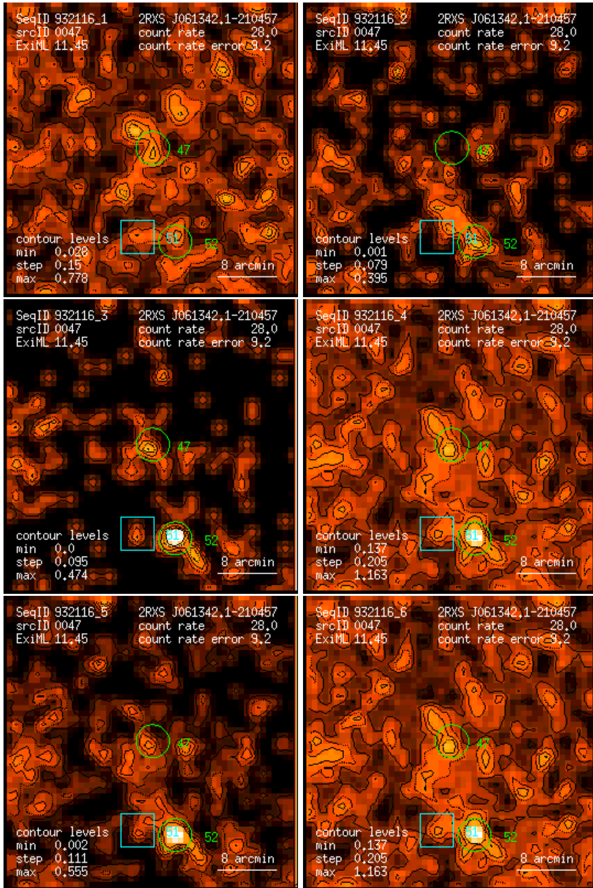
Figure 47: RASS 932116: detection 0047: band rate images, Gaussian filter: (1) PSPC channels 11 – 41, (2) 52 – 90, (3) 91 – 201, (4) 11 – 235, (5) 52 – 201, (6) 11 – 201. Broad band rates in counts/ks. Band rate contour levels in counts/ks/arcmin 2 .
