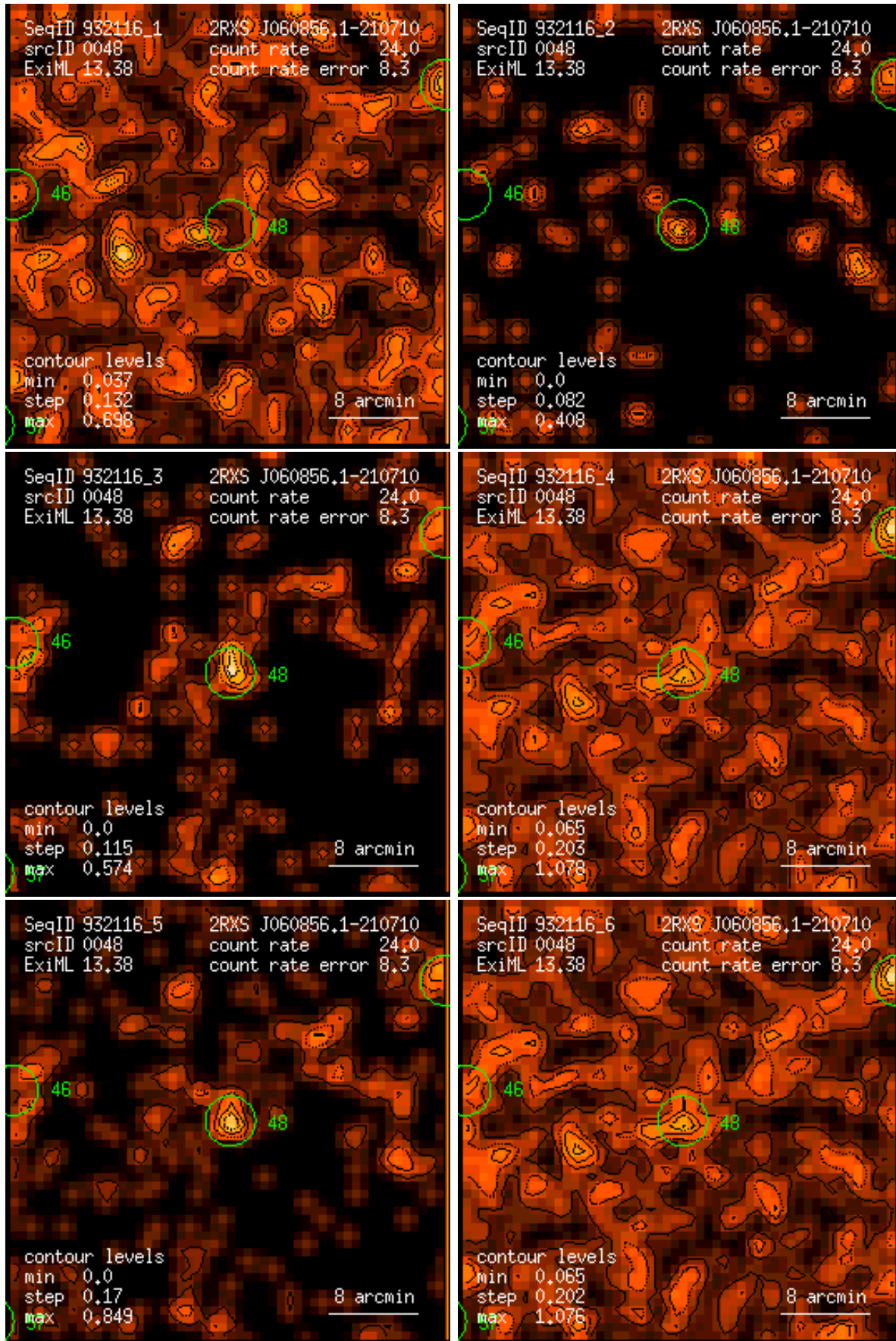
Figure 48: RASS 932116: detection 0048: band rate images, Gaussian filter: (1) PSPC channels 11 – 41, (2) 52 – 90, (3) 91 – 201, (4) 11 – 235, (5) 52 – 201, (6) 11 – 201. Broad band rates in counts/ks. Band rate contour levels in counts/ks/arcmin 2 .
