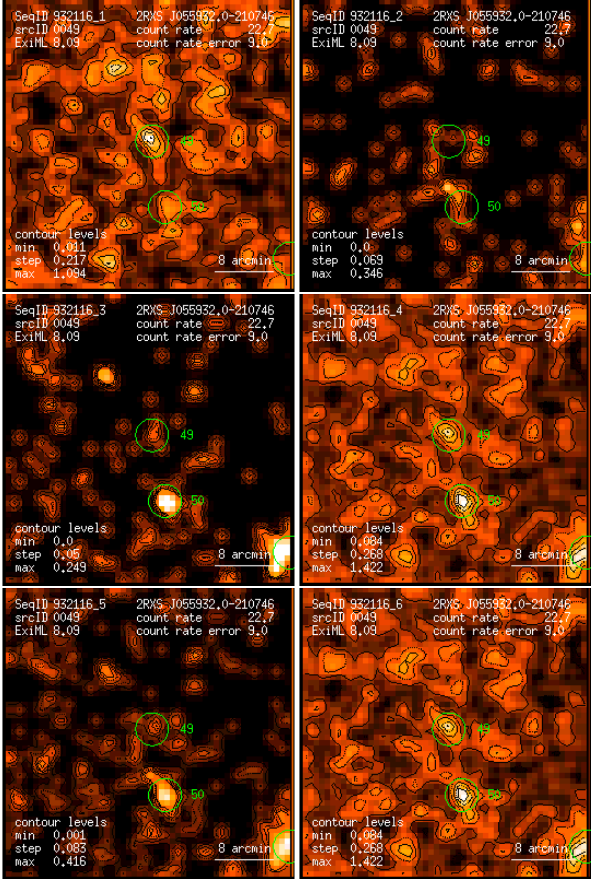
Figure 49: RASS 932116: detection 0049: band rate images, Gaussian filter: (1) PSPC channels 11 – 41, (2) 52 – 90, (3) 91 – 201, (4) 11 – 235, (5) 52 – 201, (6) 11 – 201. Broad band rates in counts/ks. Band rate contour levels in counts/ks/arcmin 2 .
