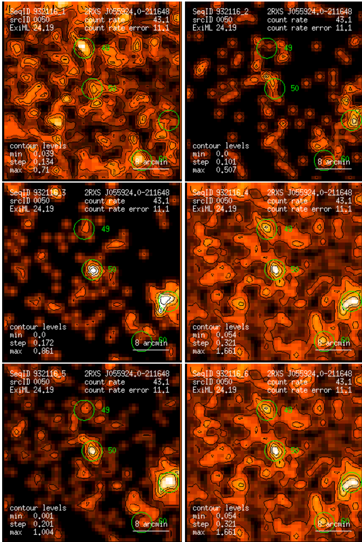
Figure 50: RASS 932116: detection 0050: band rate images, Gaussian filter: (1) PSPC channels 11 – 41, (2) 52 – 90, (3) 91 – 201, (4) 11 – 235, (5) 52 – 201, (6) 11 – 201. Broad band rates in counts/ks. Band rate contour levels in counts/ks/arcmin 2 .
