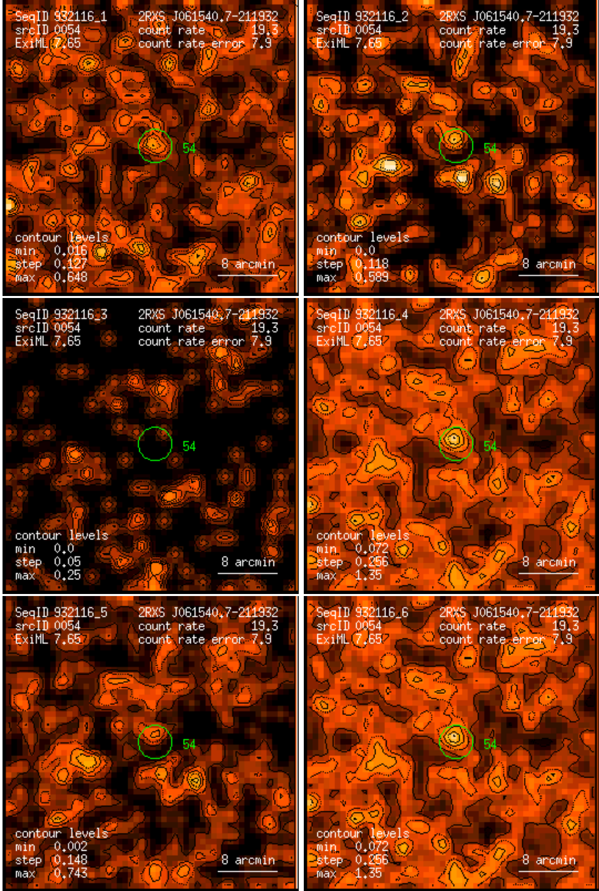
Figure 54: RASS 932116: detection 0054: band rate images, Gaussian filter: (1) PSPC channels 11 – 41, (2) 52 – 90, (3) 91 – 201, (4) 11 – 235, (5) 52 – 201, (6) 11 – 201. Broad band rates in counts/ks. Band rate contour levels in counts/ks/arcmin 2 .
