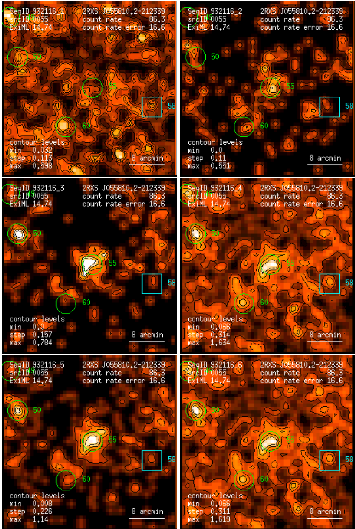
Figure 55: RASS 932116: detection 0055: band rate images, Gaussian filter: (1) PSPC channels 11 – 41, (2) 52 – 90, (3) 91 – 201, (4) 11 – 235, (5) 52 – 201, (6) 11 – 201. Broad band rates in counts/ks. Band rate contour levels in counts/ks/arcmin 2 .
