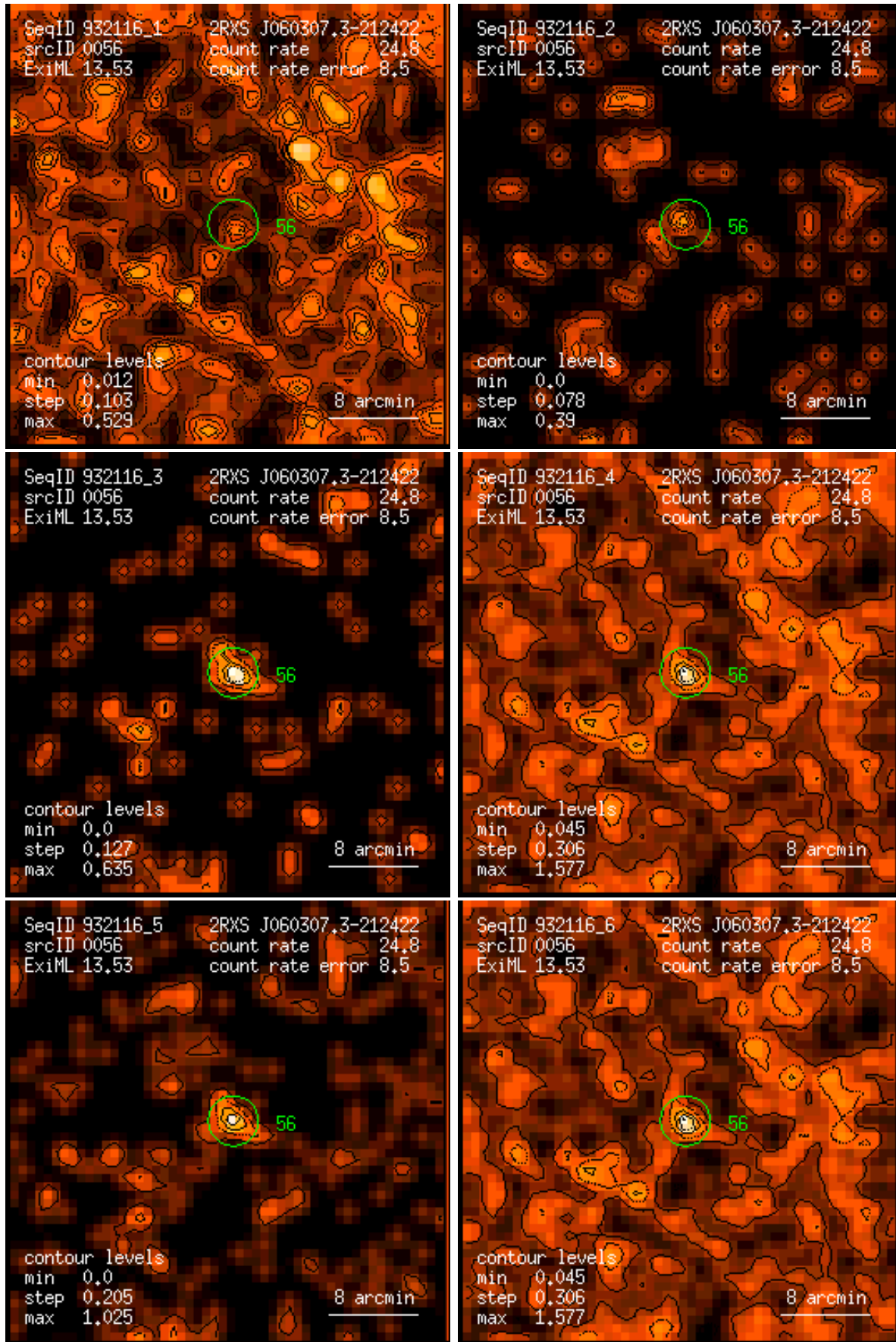
Figure 56: RASS 932116: detection 0056: band rate images, Gaussian filter: (1) PSPC channels 11 – 41, (2) 52 – 90, (3) 91 – 201, (4) 11 – 235, (5) 52 – 201, (6) 11 – 201. Broad band rates in counts/ks. Band rate contour levels in counts/ks/arcmin 2 .
