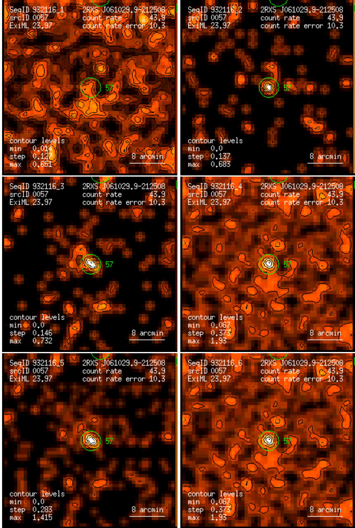
Figure 57: RASS 932116: detection 0057: band rate images, Gaussian filter: (1) PSPC channels 11 – 41, (2) 52 – 90, (3) 91 – 201, (4) 11 – 235, (5) 52 – 201, (6) 11 – 201. Broad band rates in counts/ks. Band rate contour levels in counts/ks/arcmin 2 .
