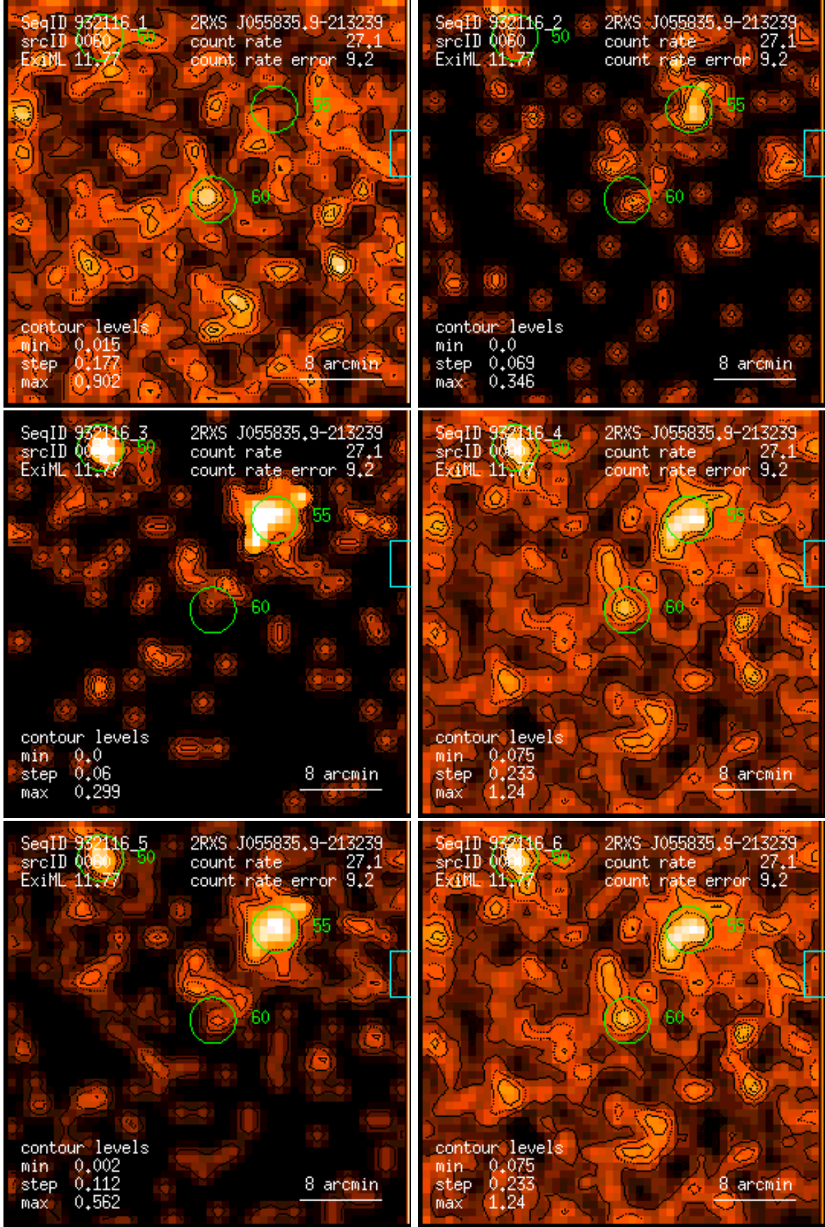
Figure 60: RASS 932116: detection 0060: band rate images, Gaussian filter: (1) PSPC channels 11 – 41, (2) 52 – 90, (3) 91 – 201, (4) 11 – 235, (5) 52 – 201, (6) 11 – 201. Broad band rates in counts/ks. Band rate contour levels in counts/ks/arcmin 2 .
