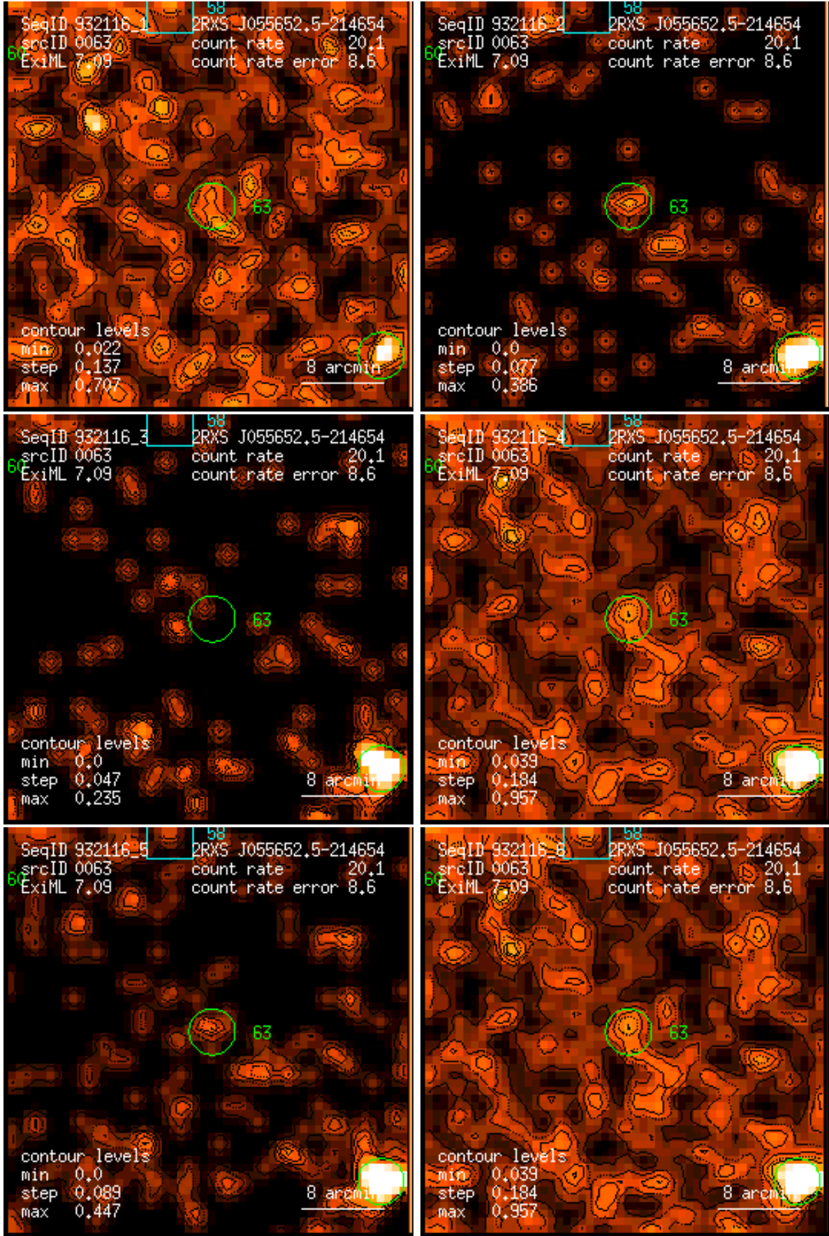
Figure 63: RASS 932116: detection 0063: band rate images, Gaussian filter: (1) PSPC channels 11 – 41, (2) 52 – 90, (3) 91 – 201, (4) 11 – 235, (5) 52 – 201, (6) 11 – 201. Broad band rates in counts/ks. Band rate contour levels in counts/ks/arcmin 2 .
