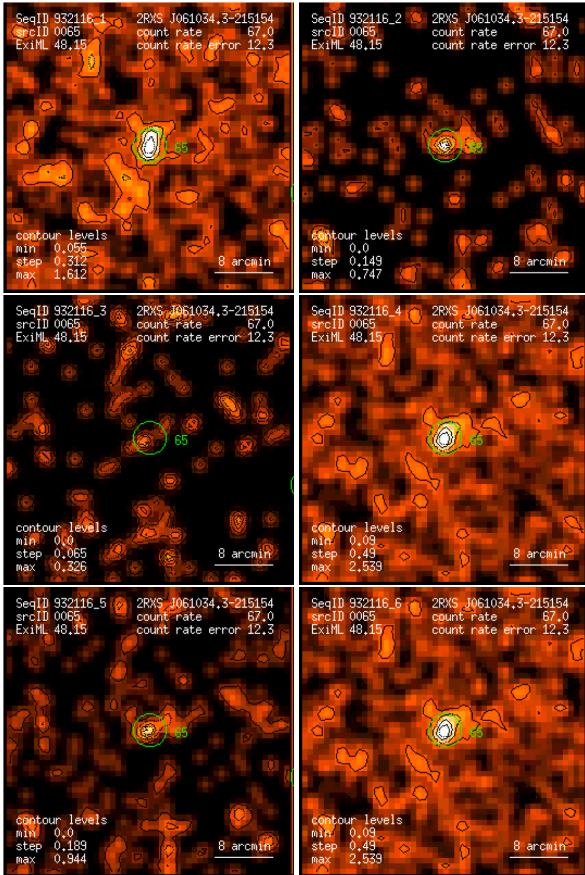
Figure 65: RASS 932116: detection 0065: band rate images, Gaussian filter: (1) PSPC channels 11 – 41, (2) 52 – 90, (3) 91 – 201, (4) 11 – 235, (5) 52 – 201, (6) 11 – 201. Broad band rates in counts/ks. Band rate contour levels in counts/ks/arcmin 2 .
