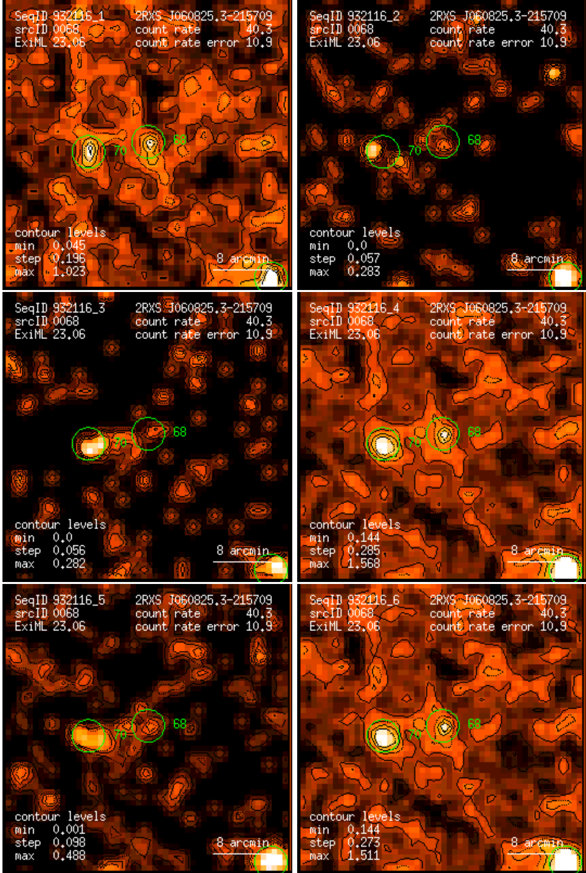
Figure 68: RASS 932116: detection 0068: band rate images, Gaussian filter: (1) PSPC channels 11 – 41, (2) 52 – 90, (3) 91 – 201, (4) 11 – 235, (5) 52 – 201, (6) 11 – 201. Broad band rates in counts/ks. Band rate contour levels in counts/ks/arcmin 2 .
