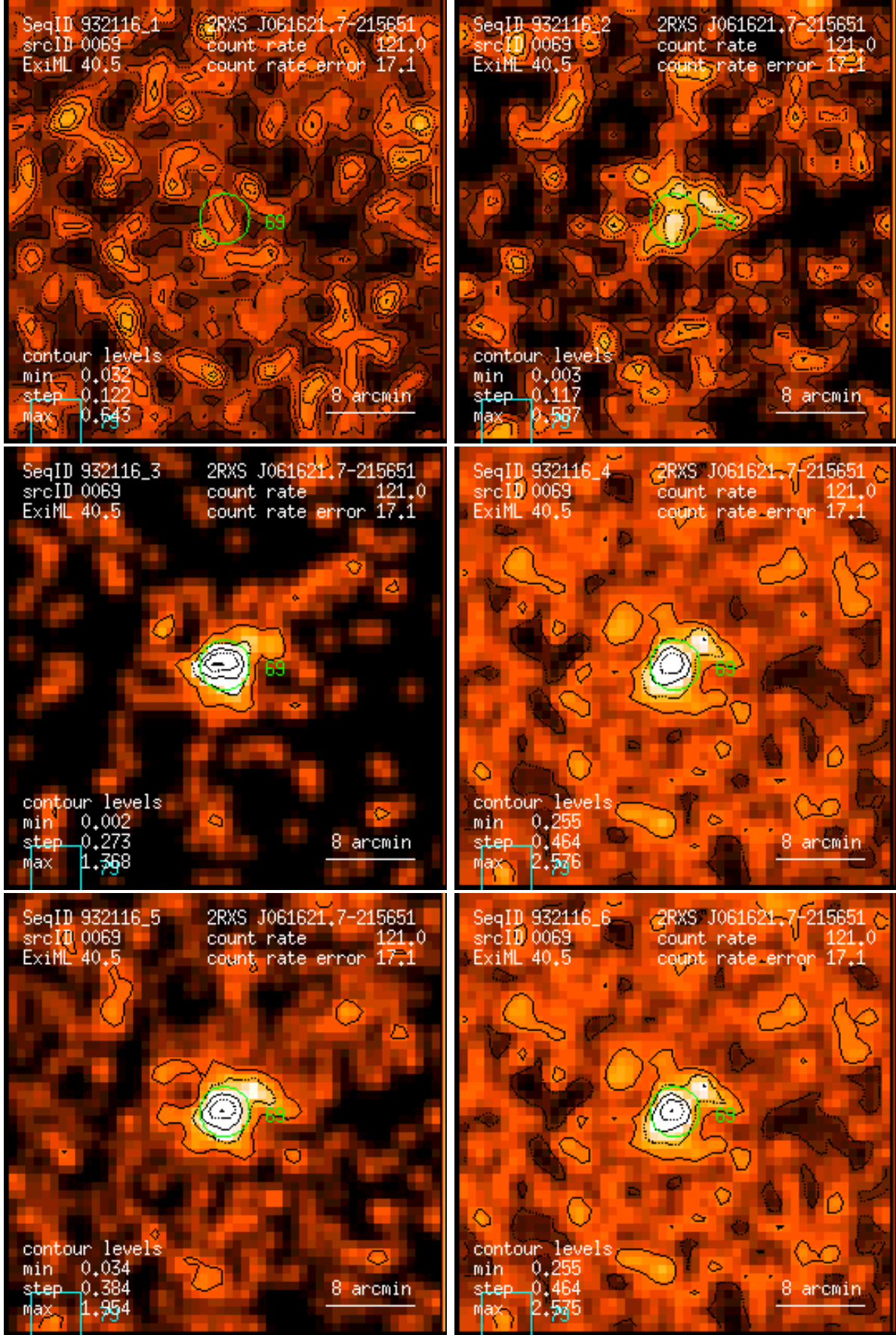
Figure 69: RASS 932116: detection 0069: band rate images, Gaussian filter: (1) PSPC channels 11 – 41, (2) 52 – 90, (3) 91 – 201, (4) 11 – 235, (5) 52 – 201, (6) 11 – 201. Broad band rates in counts/ks. Band rate contour levels in counts/ks/arcmin 2 .
