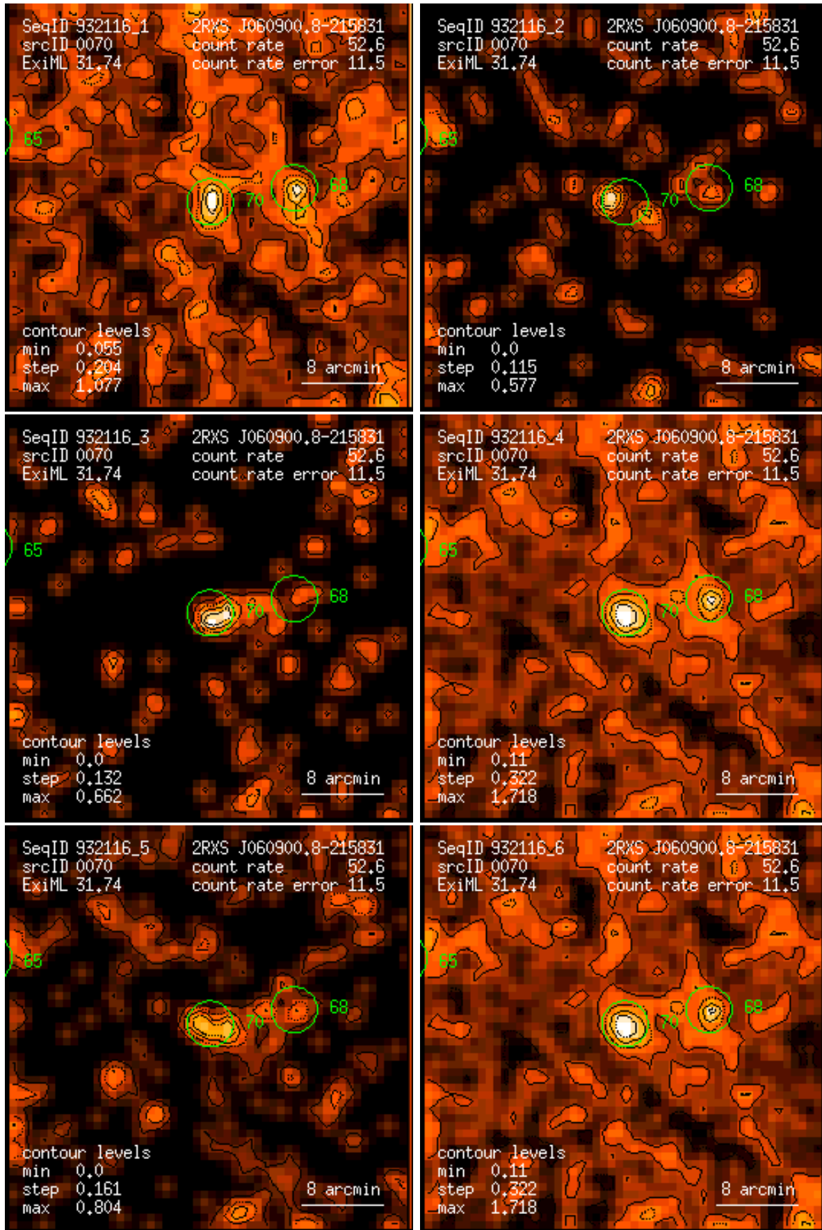
Figure 70: RASS 932116: detection 0070: band rate images, Gaussian filter: (1) PSPC channels 11 – 41, (2) 52 – 90, (3) 91 – 201, (4) 11 – 235, (5) 52 – 201, (6) 11 – 201. Broad band rates in counts/ks. Band rate contour levels in counts/ks/arcmin 2 .
