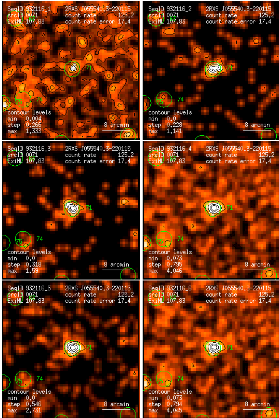
Figure 71: RASS 932116: detection 0071: band rate images, Gaussian filter: (1) PSPC channels 11 – 41, (2) 52 – 90, (3) 91 – 201, (4) 11 – 235, (5) 52 – 201, (6) 11 – 201. Broad band rates in counts/ks. Band rate contour levels in counts/ks/arcmin 2 .
