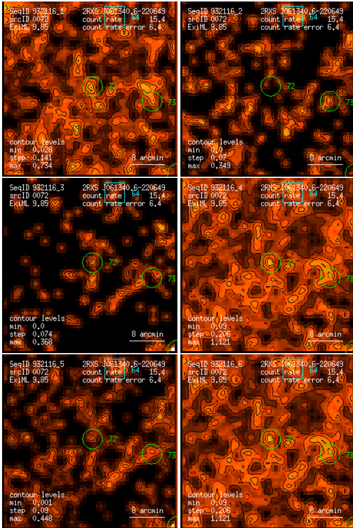
Figure 72: RASS 932116: detection 0072: band rate images, Gaussian filter: (1) PSPC channels 11 – 41, (2) 52 – 90, (3) 91 – 201, (4) 11 – 235, (5) 52 – 201, (6) 11 – 201. Broad band rates in counts/ks. Band rate contour levels in counts/ks/arcmin 2 .
