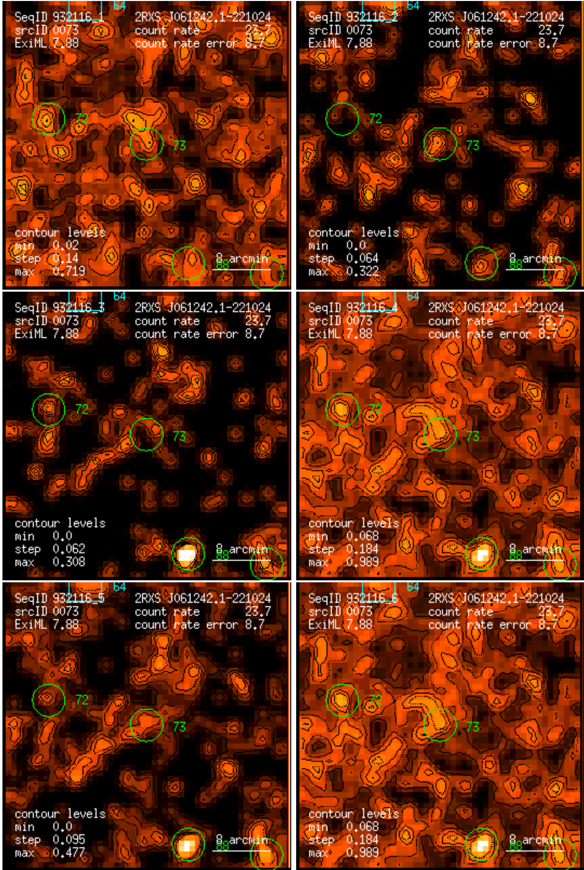
Figure 73: RASS 932116: detection 0073: band rate images, Gaussian filter: (1) PSPC channels 11 – 41, (2) 52 – 90, (3) 91 – 201, (4) 11 – 235, (5) 52 – 201, (6) 11 – 201. Broad band rates in counts/ks. Band rate contour levels in counts/ks/arcmin 2 .
