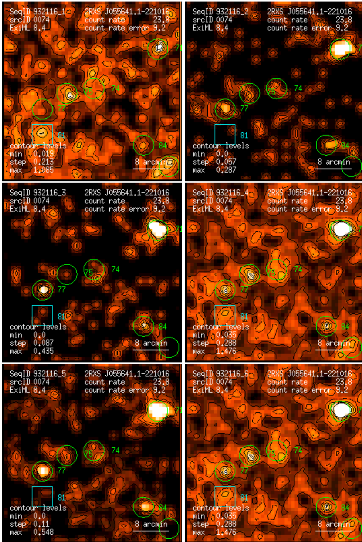
Figure 74: RASS 932116: detection 0074: band rate images, Gaussian filter: (1) PSPC channels 11 – 41, (2) 52 – 90, (3) 91 – 201, (4) 11 – 235, (5) 52 – 201, (6) 11 – 201. Broad band rates in counts/ks. Band rate contour levels in counts/ks/arcmin 2 .
