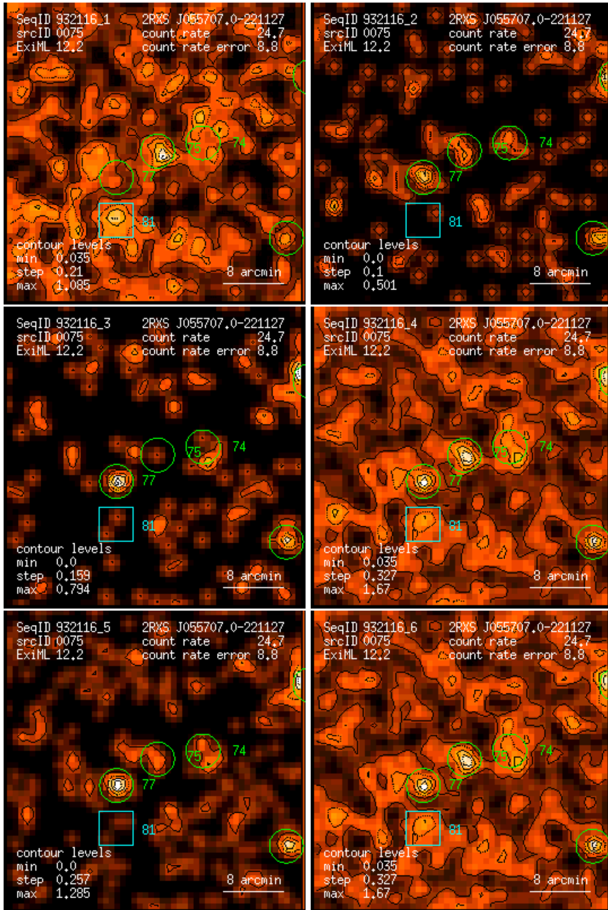
Figure 75: RASS 932116: detection 0075: band rate images, Gaussian filter: (1) PSPC channels 11 – 41, (2) 52 – 90, (3) 91 – 201, (4) 11 – 235, (5) 52 – 201, (6) 11 – 201. Broad band rates in counts/ks. Band rate contour levels in counts/ks/arcmin 2 .
