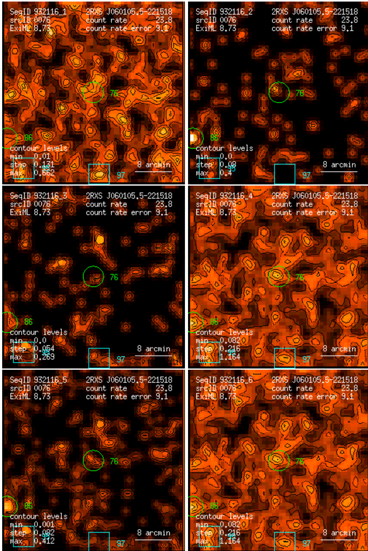
Figure 76: RASS 932116: detection 0076: band rate images, Gaussian filter: (1) PSPC channels 11 – 41, (2) 52 – 90, (3) 91 – 201, (4) 11 – 235, (5) 52 – 201, (6) 11 – 201. Broad band rates in counts/ks. Band rate contour levels in counts/ks/arcmin 2 .
