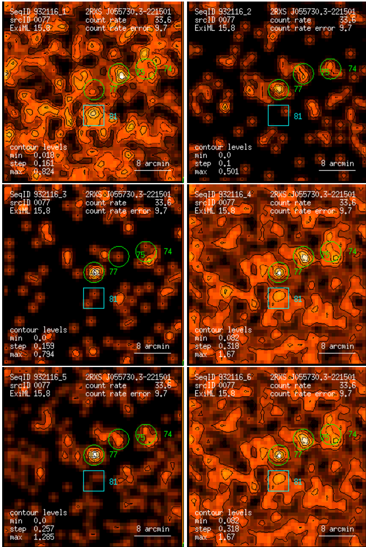
Figure 77: RASS 932116: detection 0077: band rate images, Gaussian filter: (1) PSPC channels 11 – 41, (2) 52 – 90, (3) 91 – 201, (4) 11 – 235, (5) 52 – 201, (6) 11 – 201. Broad band rates in counts/ks. Band rate contour levels in counts/ks/arcmin 2 .
