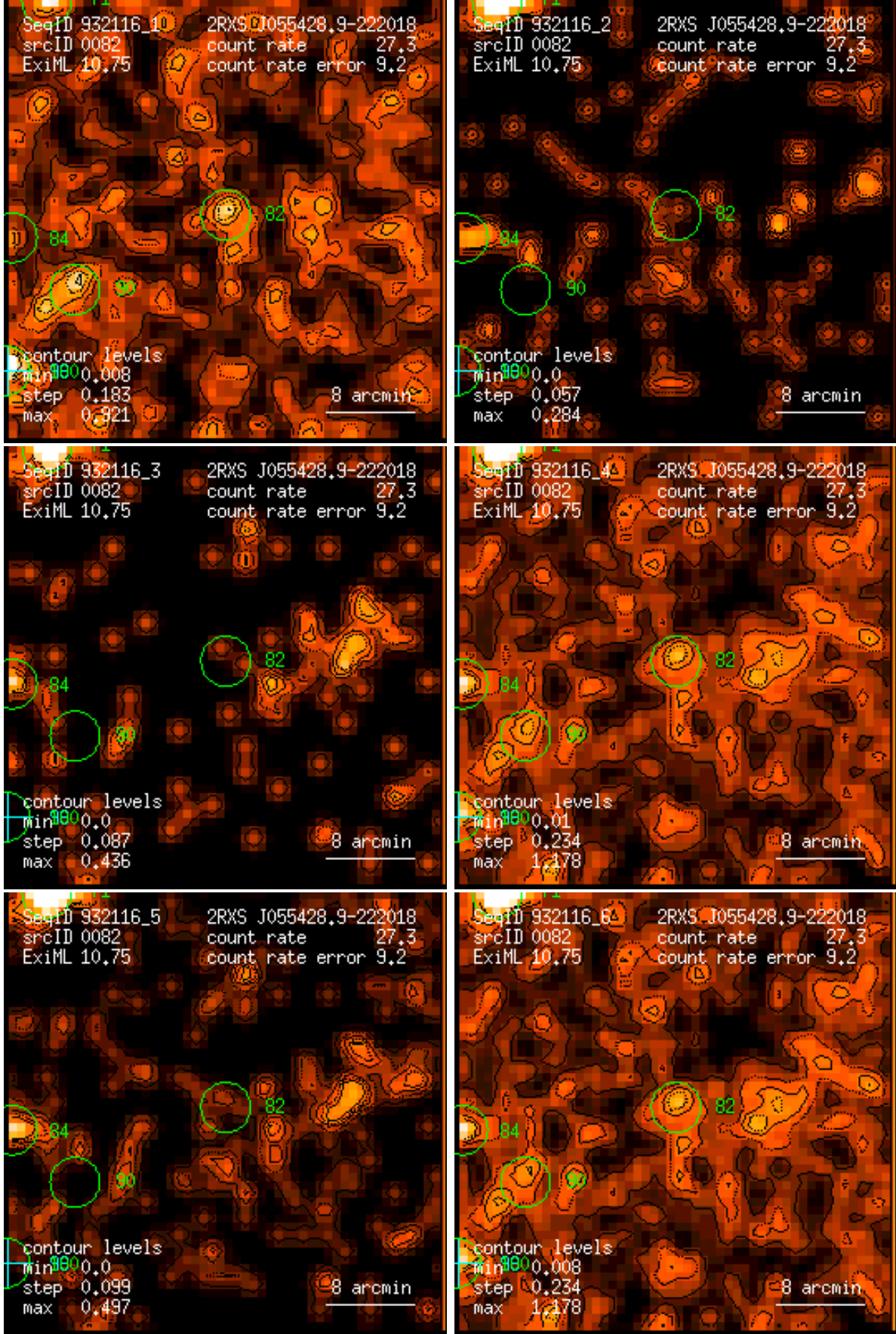
Figure 82: RASS 932116: detection 0082: band rate images, Gaussian filter: (1) PSPC channels 11 – 41, (2) 52 – 90, (3) 91 – 201, (4) 11 – 235, (5) 52 – 201, (6) 11 – 201. Broad band rates in counts/ks. Band rate contour levels in counts/ks/arcmin 2 .
