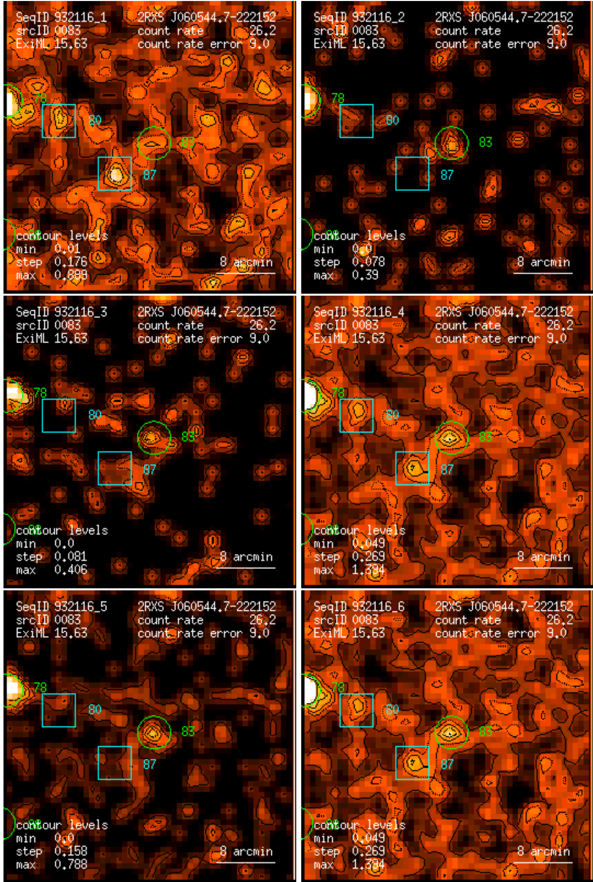
Figure 83: RASS 932116: detection 0083: band rate images, Gaussian filter: (1) PSPC channels 11 – 41, (2) 52 – 90, (3) 91 – 201, (4) 11 – 235, (5) 52 – 201, (6) 11 – 201. Broad band rates in counts/ks. Band rate contour levels in counts/ks/arcmin 2 .
