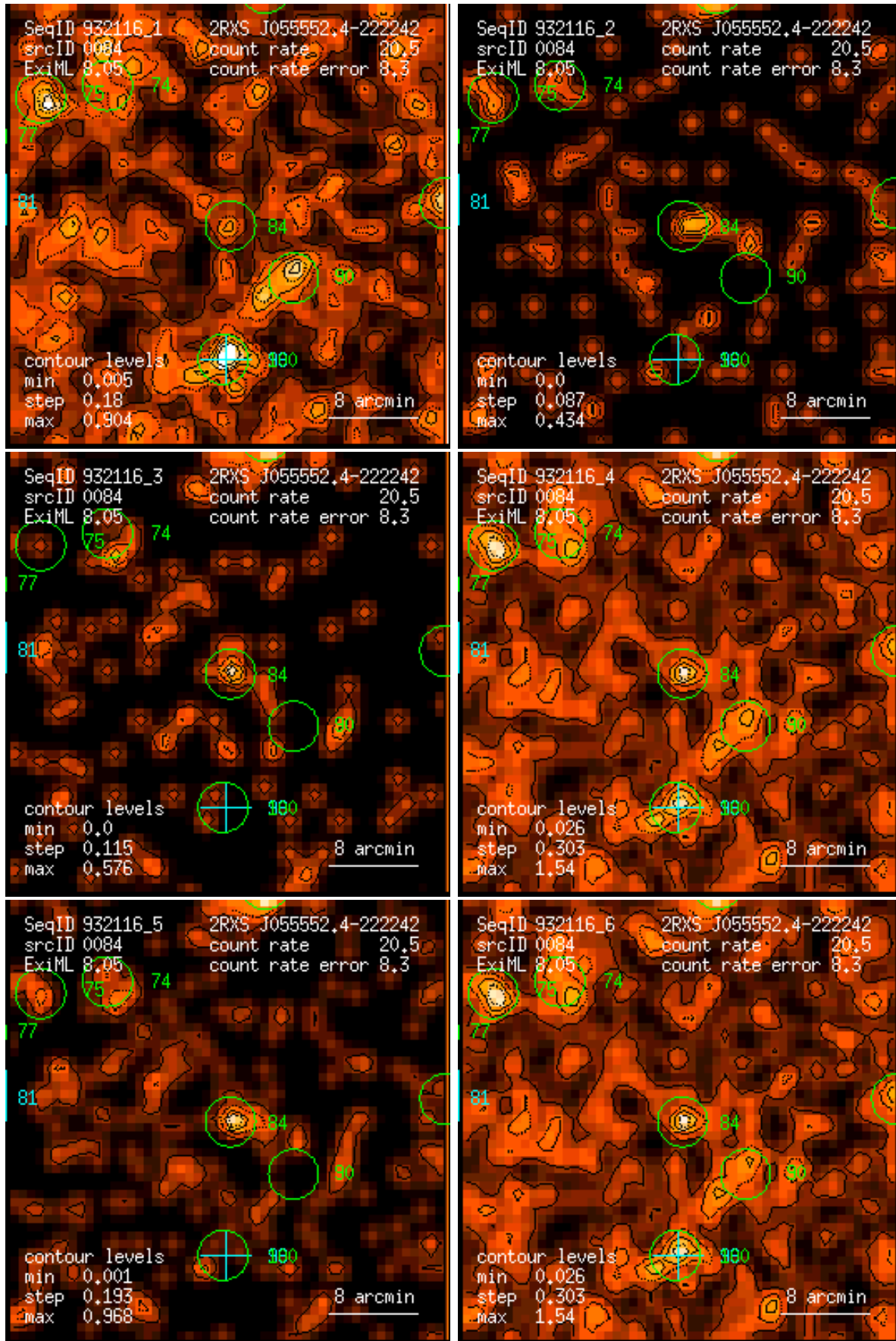
Figure 84: RASS 932116: detection 0084: band rate images, Gaussian filter: (1) PSPC channels 11 – 41, (2) 52 – 90, (3) 91 – 201, (4) 11 – 235, (5) 52 – 201, (6) 11 – 201. Broad band rates in counts/ks. Band rate contour levels in counts/ks/arcmin 2 .
