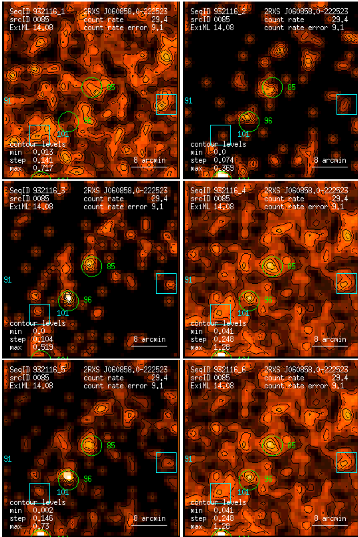
Figure 85: RASS 932116: detection 0085: band rate images, Gaussian filter: (1) PSPC channels 11 – 41, (2) 52 – 90, (3) 91 – 201, (4) 11 – 235, (5) 52 – 201, (6) 11 – 201. Broad band rates in counts/ks. Band rate contour levels in counts/ks/arcmin 2 .
