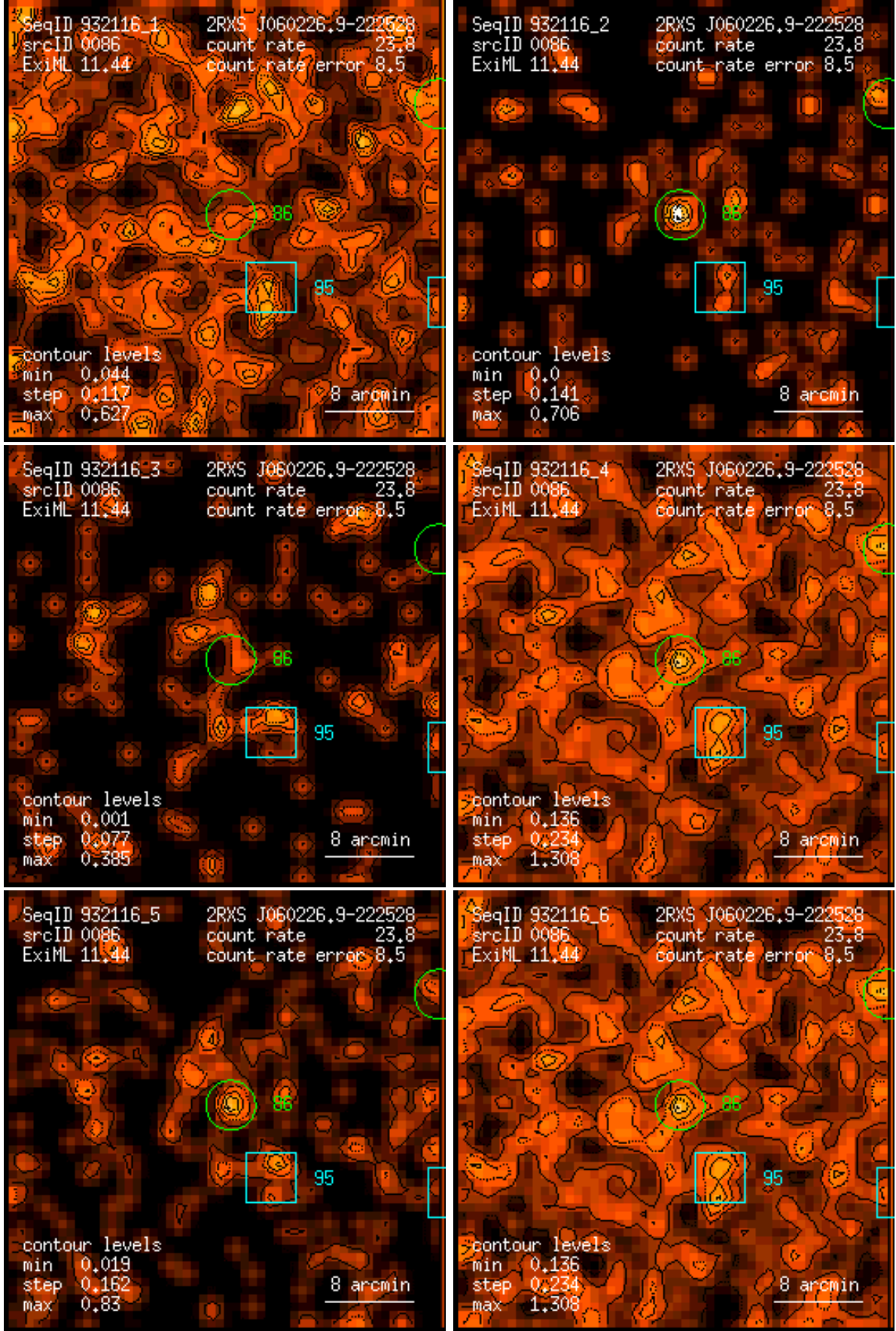
Figure 86: RASS 932116: detection 0086: band rate images, Gaussian filter: (1) PSPC channels 11 – 41, (2) 52 – 90, (3) 91 – 201, (4) 11 – 235, (5) 52 – 201, (6) 11 – 201. Broad band rates in counts/ks. Band rate contour levels in counts/ks/arcmin 2 .
